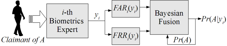
Figure 9.: Similarity scores are converted to equivalent FAR and FRR measures.
