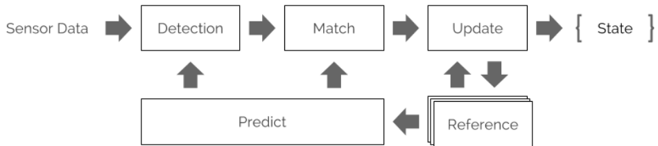
Figure 2.: Predict-match-update tracking framework
