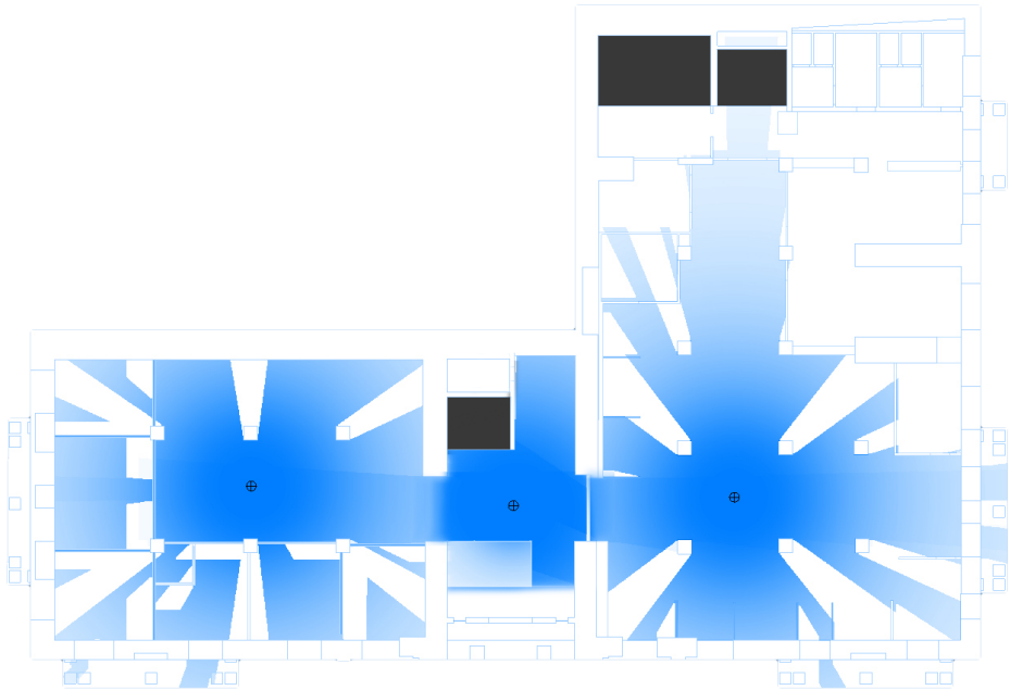
Figure 33.: Field of view of the installed CCTV cameras
