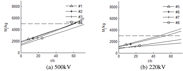
Fig.10 Ice load on transmission lines.
