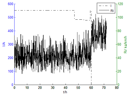
Fig.13 Current and ice accretion rate of transmission line #1.
