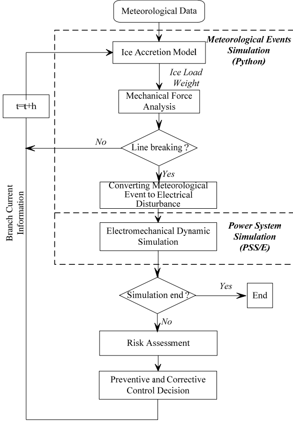
Fig.5 Hybrid simulation and control decision diagram.
