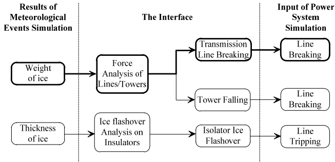
Fig. 3 Relationship between meteorological events and power system disturbances.
