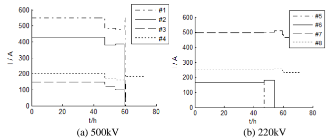
Fig.12 Current magnitudes of transmission lines during the simulation period.
