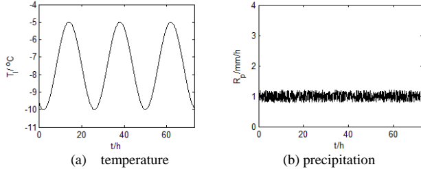
Fig.8 Ambient weather information of temperature and precipitation.
