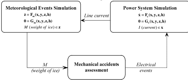
Fig. 2 Interface of the hybrid simulation scheme.
