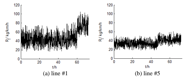
Fig.11 The time varying growth rate of ice accretion on different transmission lines.
