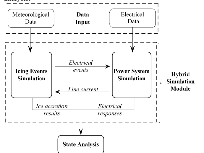
Fig.1 Hybrid simulation framework of meteorological and power systems.
