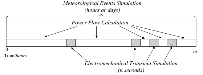
Fig. 4 Simulation time of various simulation processes.
