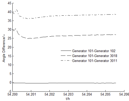
Fig.14 Angle differences between generators
