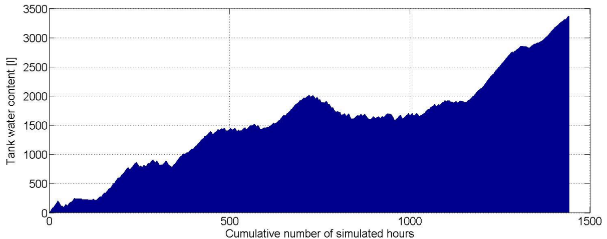
Figure 2. Seasonal profile of water stored in the tank
