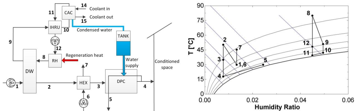
Figure 1. DDC-DWR system
