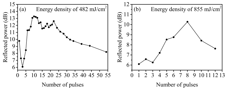
Fig. 3. Reflection of POFBG after a number of laser pulses with energy density of (a) 482 mJ/cm 2 and (b) 855 mJ/cm 2 .
