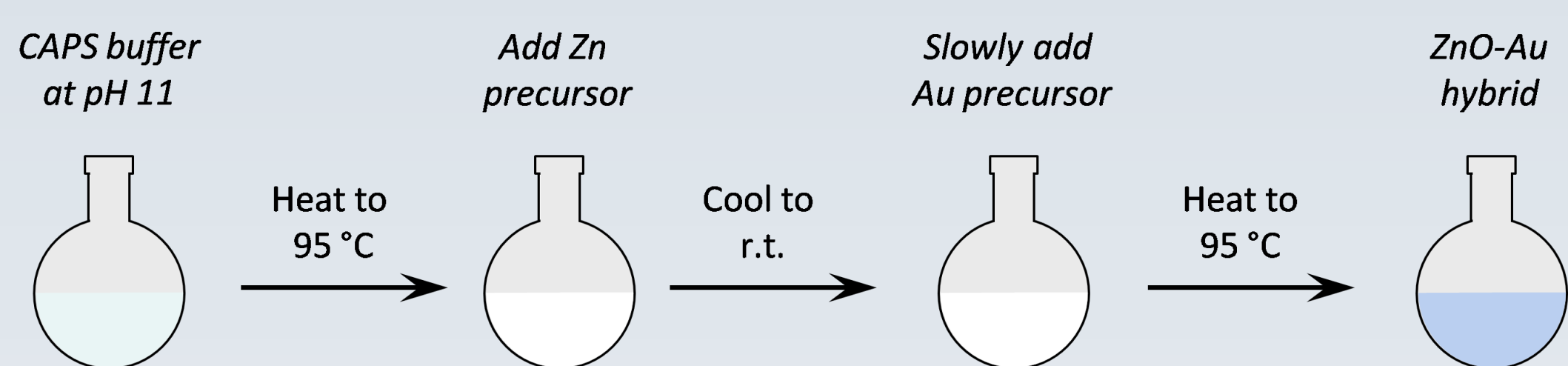
Scheme 1. Synthesis of ZnO and ZnO-Au hybrids. N -cyclohexyl-3-aminopropane-sulfonic acid (CAPS) buffer is adjusted to pH 11 and heated to 95 °C before addition of Zn precursor solution. After formation of ZnO, the mixture is cooled and HAuCl 4 is added dropwise. Finally, the mixture is heated again reducing the Au precursor forming ZnO hybrids.
