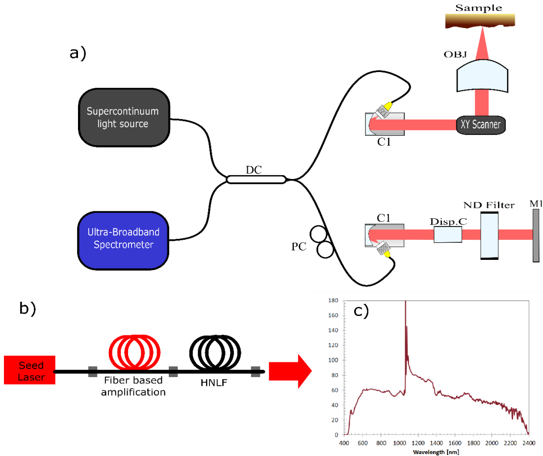
Fig. 1: System description: (a) Schematic of the UHR-OCT system with DC: directional coupler, C1: collimators, PC: polarization controller, XY scanner a pair of galvo-scanners, OBJ: objective, Disp.C: dispersion compensation block, ND Filter: neutral density filter, M1: flat mirror. (b) Typical SC design. (c) Example of SC output spectrum.
