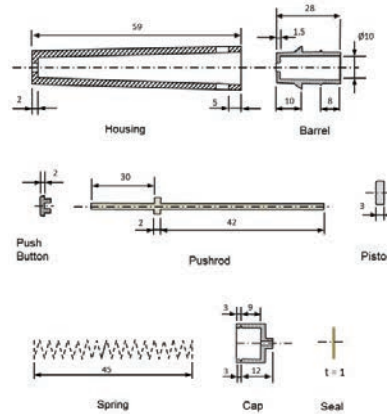
Fig 6 Dimensions related to study of each part
