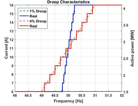
Fig. 4. The droop characteristics for the controller.
