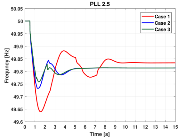
Fig. 10. The frequency at bus 2.5 with different delays in the EVs model.
