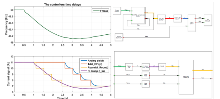
Fig. 5. The control process by the controller.
