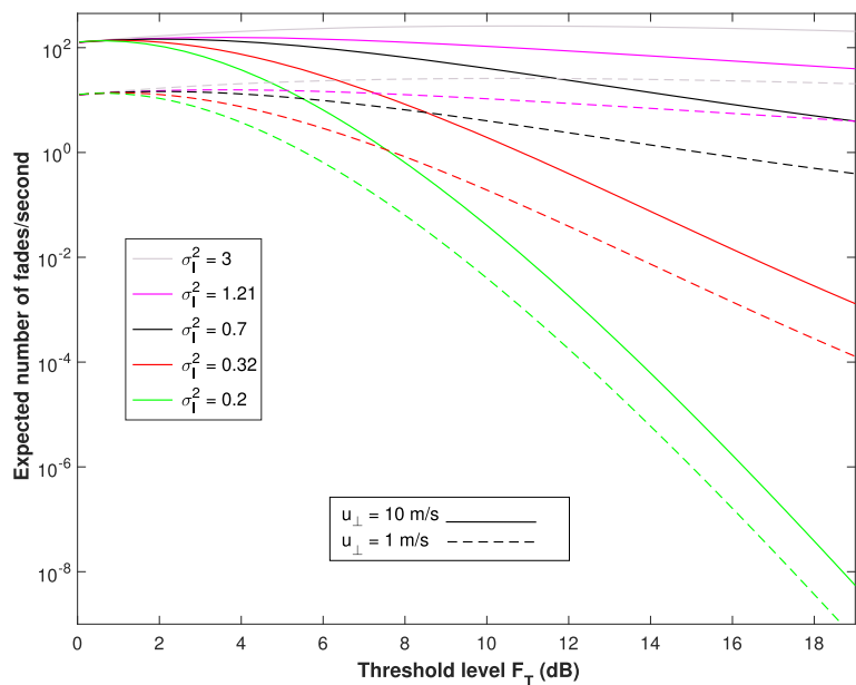
Fig. 3 Expected number of fades versus F_T = 10 \cdot \log_{10}(\frac{\langle I \rangle}{I_0}) for a Málaga turbulence model for two different crosswind speeds: u_{\perp} = 1 and u_{\perp} = 10 m/s. Turbulent channel parameters (\alpha, \beta, \Omega, \rho) were taken from Table 1
