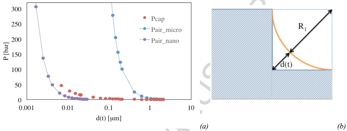
Figure 12 Capillary pressure ( P_{cap} ) and pressure due to the trapped air, for micro and nano-features ( Pair ), at 150^{\circ}\text{C} , versus the decrease of the filling distance d(t) calculated from equation 6 and 4 respectively (a). A sketch of the feature is also reported (b).
