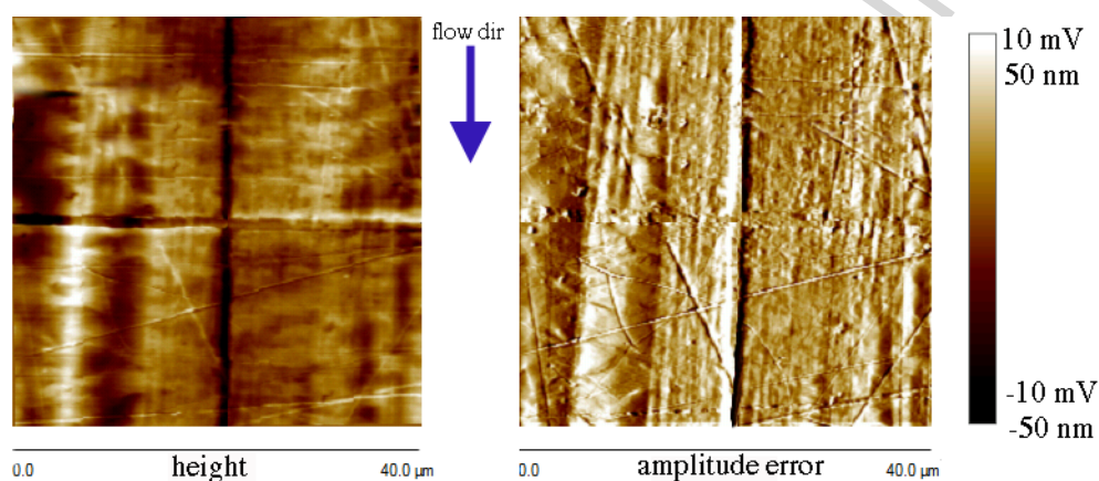
Figure 15 AFM height map and AFM amplitude error (from left to right) of the nano-feature on the sample obtained with T_{\text{level}}=150^{\circ}\text{C} , t_{\text{h}}=13 s and P_{\text{h}}=360 bar. The flow direction is also reported.
