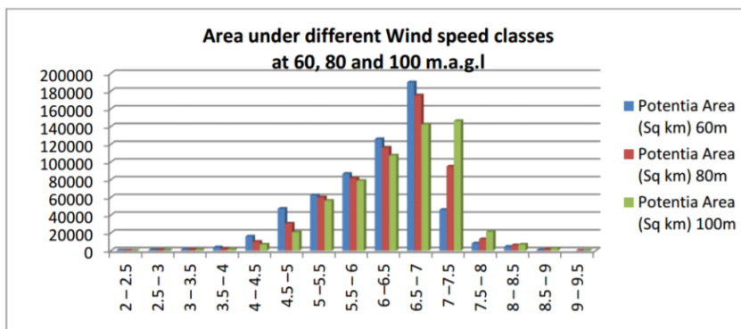
Figure 11: Comparative Analysis of Wind speed at 60m, 80m and 100m, (GoK Ministry of Energy and WinDForce, 2013)
