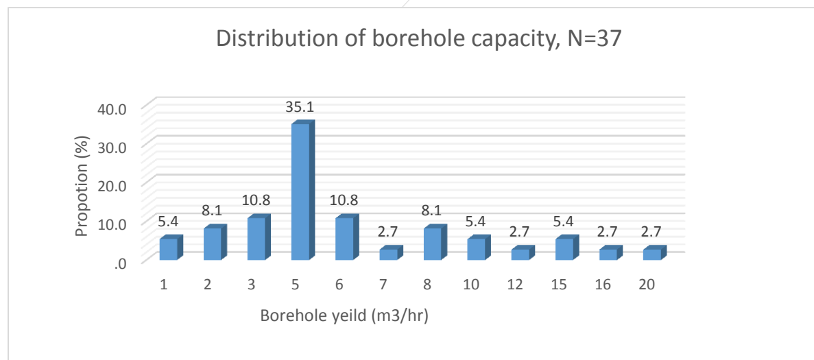
Figure 20: Distribution of safe borehole yield
