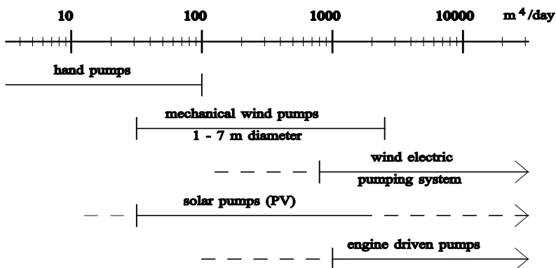
Figure 10: The wind pumping niche versus other pumping
