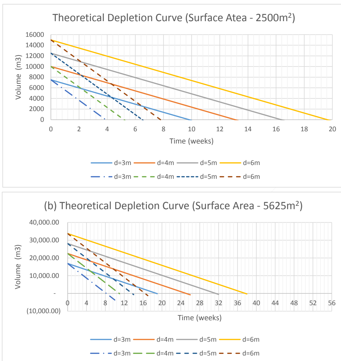
Figure 21: Theoretical depletion curves without irrigation
