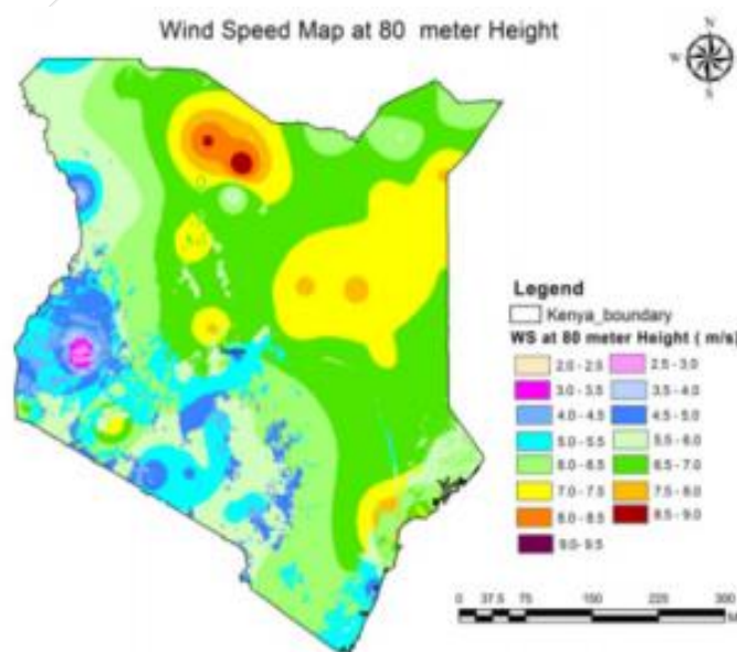
Figure 9: Wind Speed Map of Kenya at 80m height
