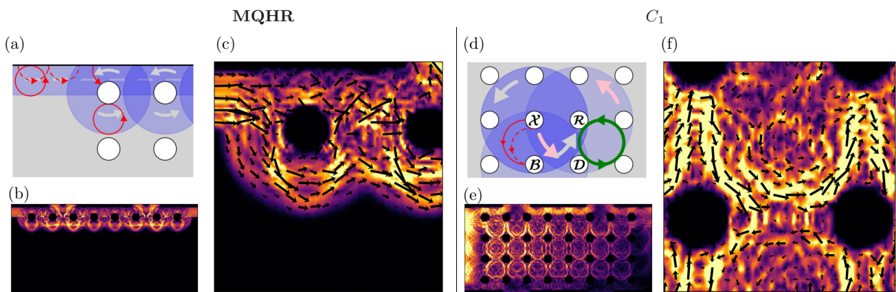
FIG. 3. Schematics and current maps for the modified quantum Hall (MQHR) and first commensurability peak ( C_1 ) regimes. (a,d) Schematics showing the extent of edge and/or ring states (blue shaded areas) in the given regime, net current flow directions (gray, pink arrows), and individual semiclassical trajectories (red dashed and solid lines). The thicker green circle in (d) shows the expected size of the 1a type pinned orbit at this magnetic field value. (b,e) Current heat maps of the entire device. (c,f) Zoomed region of heat maps in (b,e) with current flow directions illustrated by arrows.
