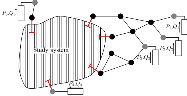
Fig. 4. DPIs are placed at each boundary bus.
