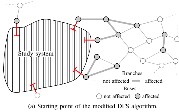
Fig. 3. Visualization of buffer zone identification.
