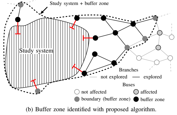
Fig. 3. Visualization of buffer zone identification.
