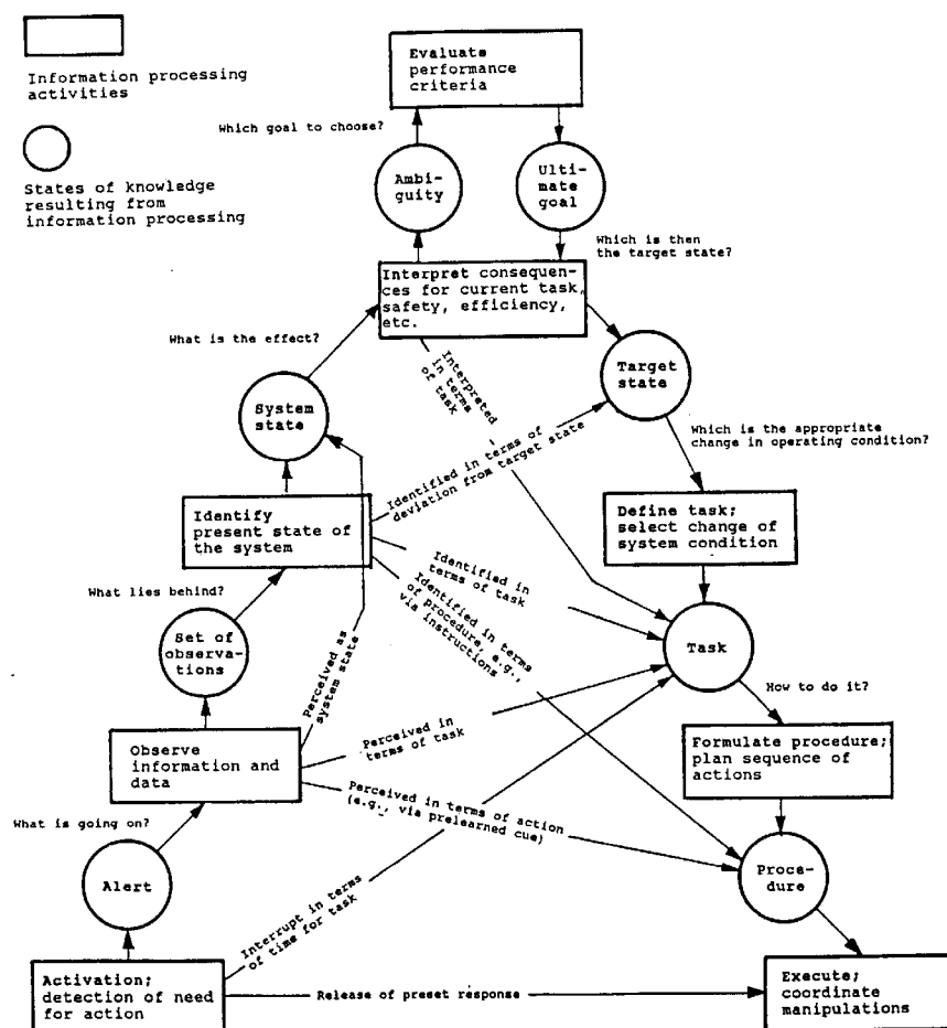
Figure 2. Schematic map of the sequence of information processes involved in a control decision. Rational, causal reasoning connects "states of knowledge" in the basic sequence. Stereotyped processes based on "know-how" can by-pass intermediate stages.
