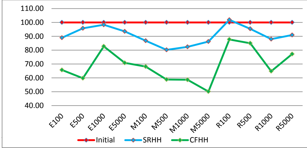
Figure 5: Compactness of solutions generated by FTF, and following improvement by CFHH and SRHH
