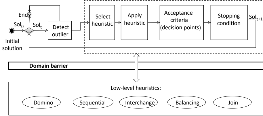
Figure 2: Proposed perturbative selection hyper-heuristic framework
