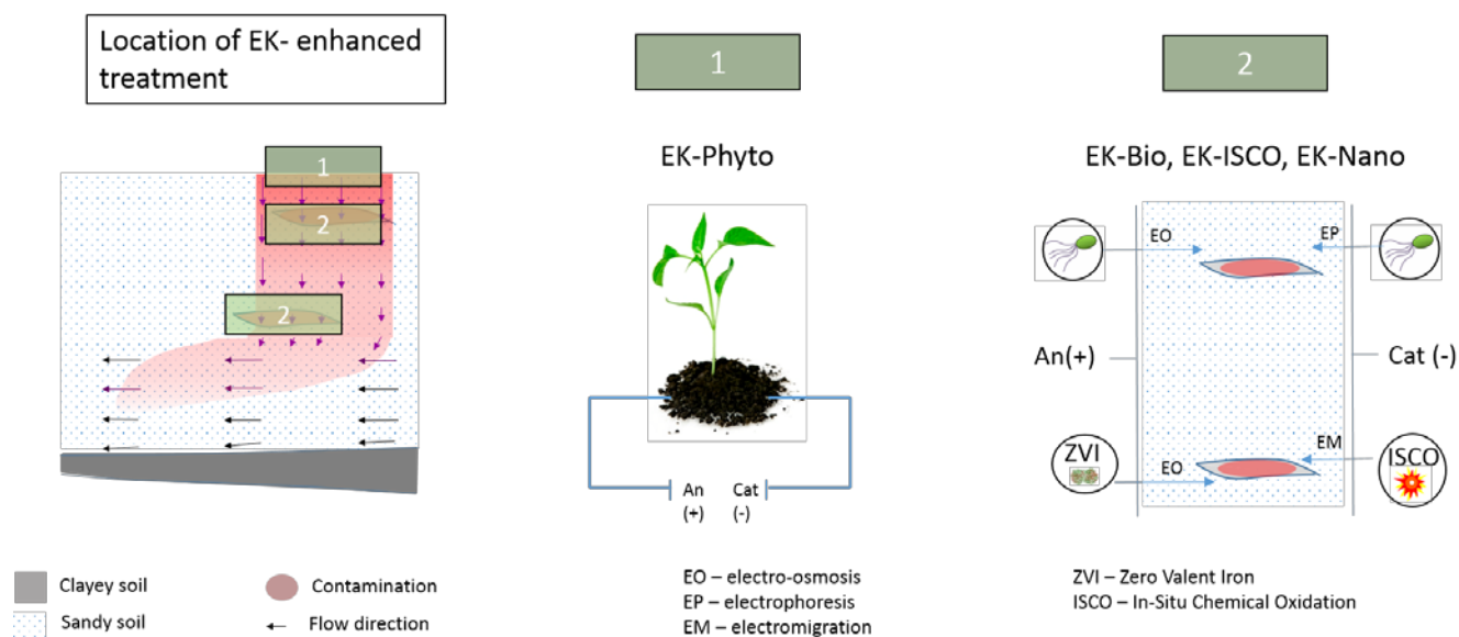
Figure 2 – Schematic representation of electrokinetically enhanced remediation. The left most scheme shows where, within the subsurface or underground, which EK-enhancement would be better suited. Scheme 1 (middle frame) represents the combination of EK with phytoremediation. Scheme 2 (right frame) summarizes how EK would enhance/transport/aid bioremediation, ISCO and nZVI applications.
