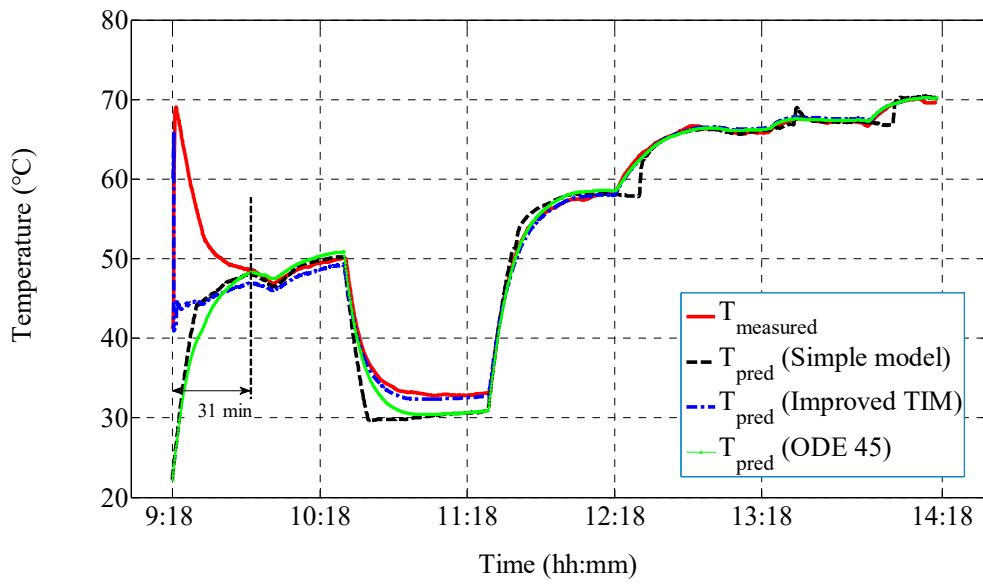
Figure 7 Comparisons of the collector outlet temperature predictions by different solution models with the measured data. Simple model – the simple dynamic model based on the piston flow concept; Improved TIM – The improved thermal inertia model of flat-plate solar collectors based on the two-node lumped heat capacitance (Deng et al., 2016a); ODE 45 – the prediction of the fourth-order numerical solution of Equation (15) using the ode45 solver in Matlab
