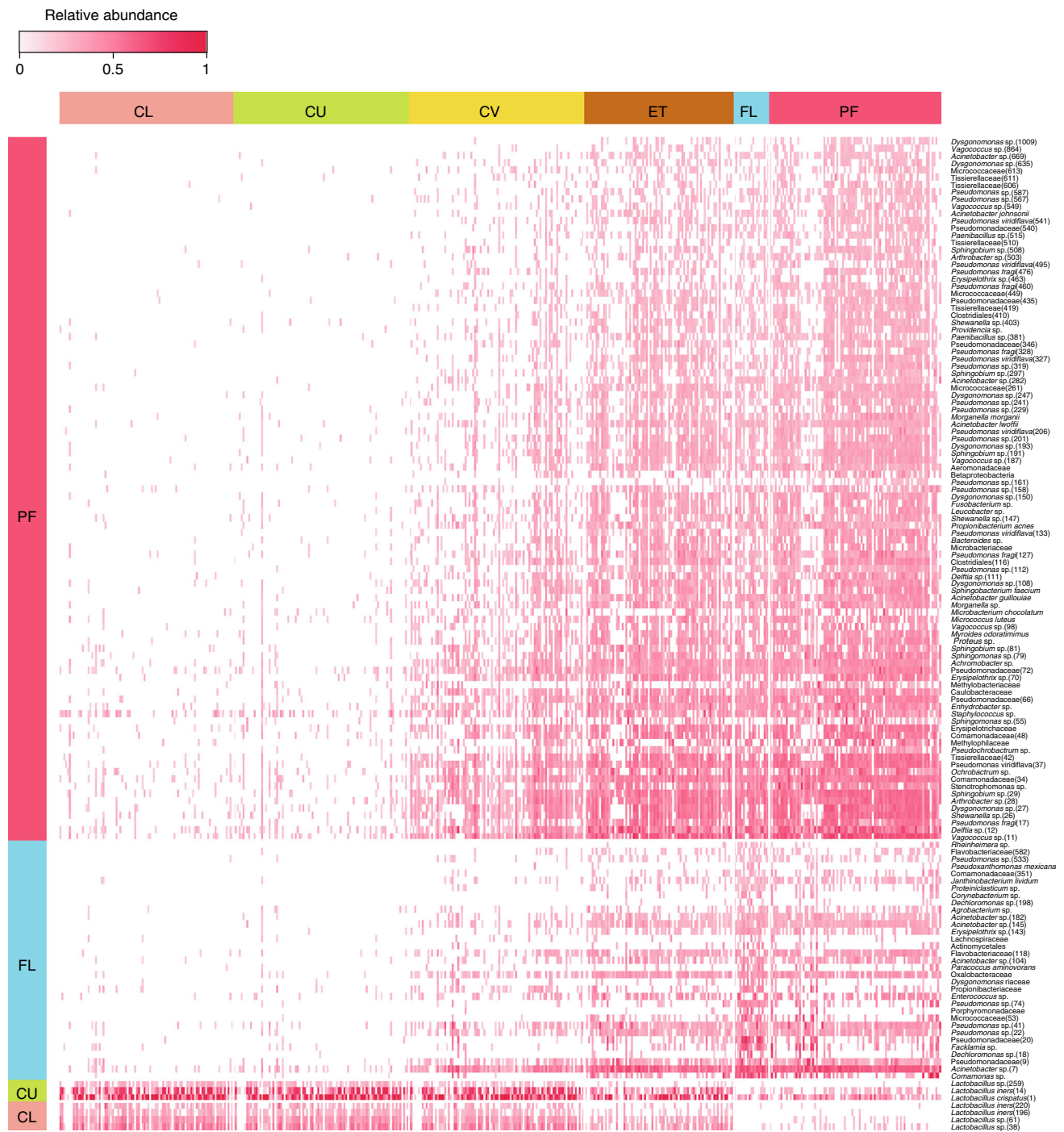
Fig. 2 Signature species for each body site. Heatmap for the relative abundances of signature OTUs from each body site ( P < 0.05 , multi-level pattern analysis, and IndVal > 0.5 ). Each bar represents one sample ( n = 94 CL, 95 CU, 95 CV, 80 ET, 93 PF, 9 FLL and 10 FRL, Supplementary Data 1)
