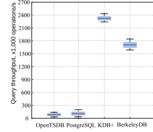
Fig. 6. Throughput of querying small data set
