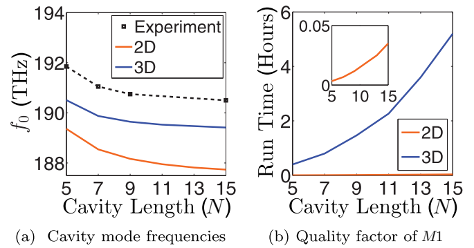
FIG. 2. Passive cavity simulations for an LN cavity in a triangular PC cavity with lattice pitch a = 438 nm, radius r = a/4 , height h = 250 nm (in 3D), and refractive index n = 3.17 or 2.54 for 3D and 2D simulations, respectively. (a) Comparison of the fundamental mode's peak frequency as a function of cavity length, for 2D and 3D simulations, with experimental data points from [13] for reference. (b) Run-time requirements using 16 cores with 1024 Mb of memory, for a single passive 2D or 3D simulation, without QD mesh requirements, as a function of cavity length (see text).
