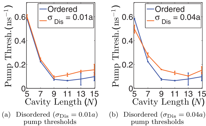
FIG. 16. Pump threshold trends for two disordered simulations: intrinsic levels \sigma_{\text{Dis}} = 0.01a (a), and larger than intrinsic disorder \sigma_{\text{Dis}} = 0.04a (b), demonstrating a general increase in the pump threshold predominantly for cavity lengths greater than L7 .
