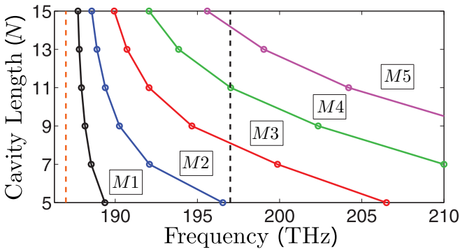
(a) Cavity frequencies versus length
