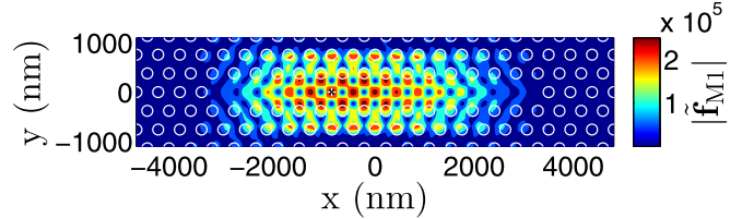
(c) Disordered ( \sigma_{\text{Dis}} = 0.01a ) cavity mode profile, f_2 above
