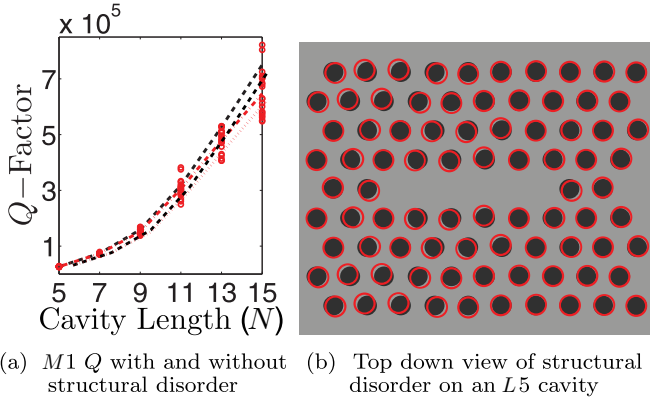
FIG. 3. (a) Impact of intrinsic levels of structural disorder (red circles) on 3D FDTD PC cavity simulations as a function of cavity length, averaged over 20 instances (red dotted-dashed line), compared to ordered simulations (dashed black line). (b) Schematic top view of the disordered cavity simulation with the disordered holes (red circles) over-top the ideal air holes (black holes), and the background slab (gray); this is a zoom-in region and in the simulations use a larger domain seen in Fig. 5(b).
