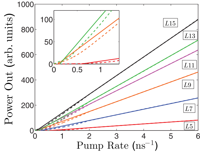
FIG. 10. Example lasing curve, or LL graphs of the \omega_1 QD ensemble, where the dashed lines represent simulated data, and solid lines are the linear fit used to extract pump threshold. The inset is a closeup of the L5 , L9 , and L13 curves.
