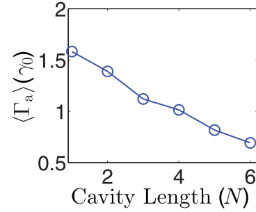
FIG. 15. Total ensemble average of the single QD radiative decay rate for each LN cavity averaged over 50 statistical variations of each instance shown in Fig. 14. In contrast to the peak Purcell factor trends, we clearly see a decrease in the average radiative decay rate for increasing cavity lengths that would be randomly sampled by the QDs.
