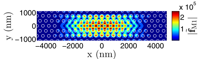
(b) Ordered cavity mode profile, f_1 above
