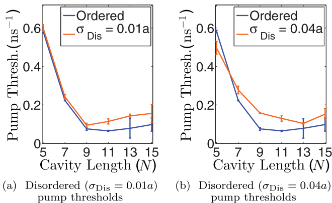
FIG. 16. Pump threshold trends for two disordered simulations: intrinsic levels \sigma_{Dis} = 0.01a (a), and larger than intrinsic disorder \sigma_{Dis} = 0.04a (b), demonstrating a general increase in the pump threshold predominantly for cavity lengths greater than L7 .
