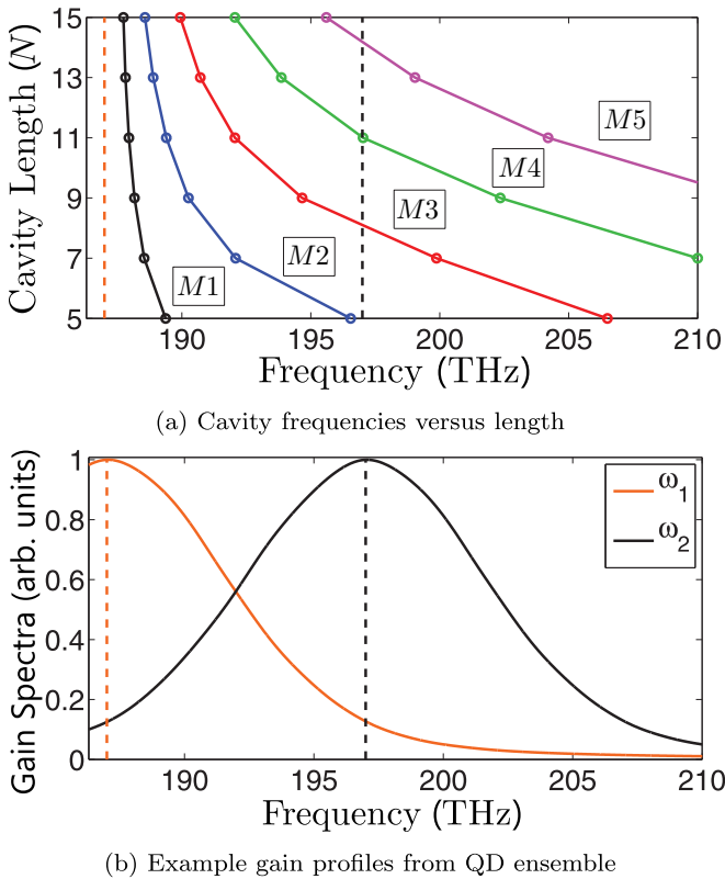
FIG. 8. (a) Dependence of the cavity mode peak frequencies, for each cavity length, to the resonant peak QD ensemble gain (or PL) spectra. (b) Visualization of the normalized inhomogeneously broadened gain spectra of the QD ensemble for \omega_1 (gain model A) and \omega_2 (gain model B) taken from Fig. 6(a).
