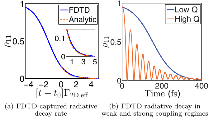
FIG. 7. (a) Population \rho_{11} dynamics within an L5 low- Q -factor ( \approx 400 ) cavity, solved by MBE without any decay terms, so all phenomenological decay parameters are set to zero and the radiative decay is captured self-consistently through the local electric field used in the OBE solver. The OBEs are given initial conditions \rho_{11}(t=0) = 0.95 , \rho_{01}^{\text{im}}(t=0) = 0 , and \rho_{01}^{\text{re}}(t=0) = \sqrt{1 - 0.95^2}/2 , such that the Bloch vector magnitude is set to unity (e.g., \sigma_1 = 2\rho_{11} - 1 , \sigma_2 = 2\rho_{01}^{\text{re}} , and \sigma_3 = 2\rho_{01}^{\text{im}} are the usual Bloch vector components with magnitude \sigma_1^2 + \sigma_2^2 + \sigma_3^2 ). The analytic solution is determined by \Gamma_{2D, \text{eff}} , calculated by the QNM GF seen in Fig. 6(b). (b) Comparison of high- and low- Q cavities for the 2D L5 cavity structure, which were 47000 and 430, respectively. All other parameters are the same as in (a).
