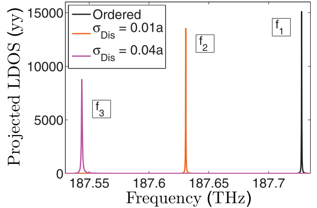
(a) L15 cavity LDOS for ordered, and disordered M1 modes
