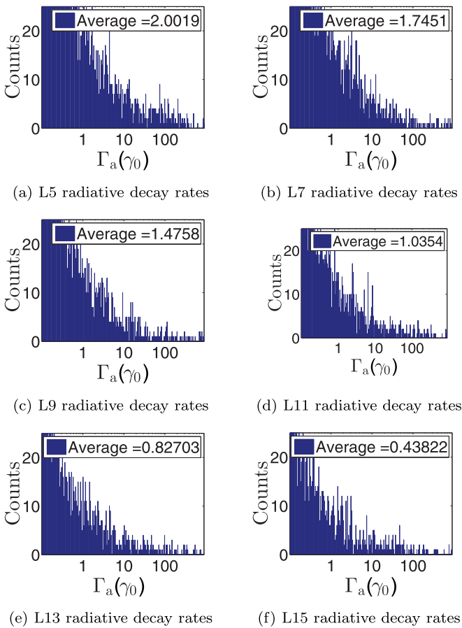
FIG. 14. For each cavity length, we show an example instance of the bar-graph statistics from 300 bins of the single-position radiative decay rates overlapping with the fundamental ( M1 ) cavity mode, where the center frequencies of the dipole emitters are randomly assigned as before. The total average enhancement rates for each statistical distribution, using all spatial points in the spatial mode active region, is shown in each panel (in units of \gamma_0 ).
