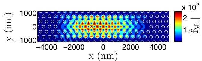
(c) Disordered ( \sigma_{Dis} = 0.01a ) cavity mode profile, f_2 above
