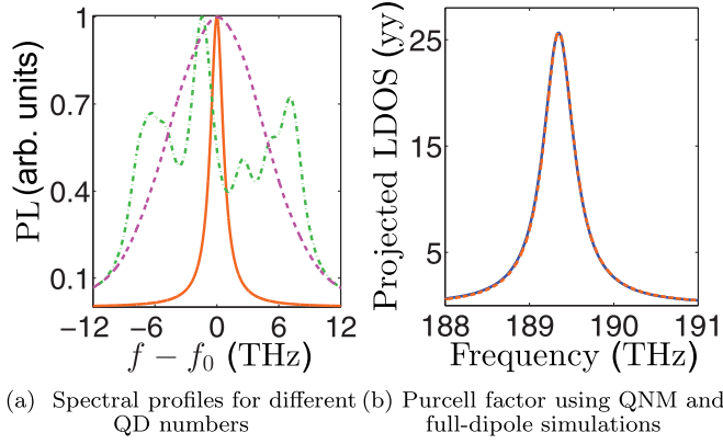
FIG. 6. (a) Modeled QD ensemble (dashed and dotted-dashed lines) for 10 (green chain) and 10000 (magenta dashed line) QDs, for typical room-temperature inhomogeneous broadening. The individual QD line shape is given by the orange (light) line, with \gamma' = 1.5 THz. The y -shows a normalized photoluminescence (PL) for individual (solid line) and ensembled (dashed or dotted-dashed lines) QDs. The number of QDs in each simulation is on the order of 10000. (b) Fundamental mode comparison between full-dipole expansion (blue line) and QNM theory (orange dashed line) for low- Q cavity, with a reduced PC membrane. The projected LDOS has been normalized to represent PF.
