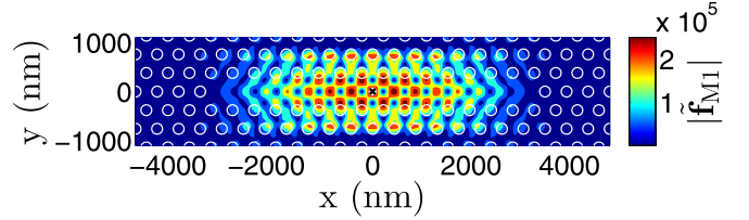
(b) Ordered cavity mode profile, f_1 above
