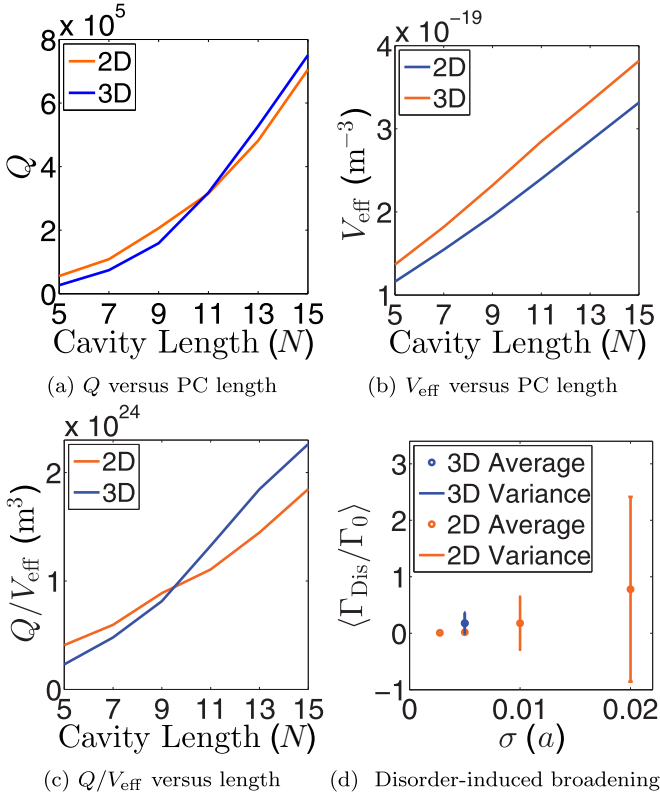
FIG. 4. (a)–(c) Q and V_{\text{eff}} modeling of effective 2D system compared to full 3D simulations, without disorder. (d) Disorder statistics of \Gamma_{\text{Dis}} = \Gamma - \Gamma_0 , for the L15 cavities of varying amounts of 2D disorder, referenced to the 3D intrinsic disorder of \sigma_{\text{Dis}} = 0.005a .
