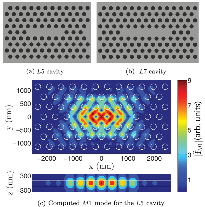
FIG. 1. Top-down view region of an L5 (a) and L7 (b) PC slab cavity. (c) First fundamental mode ( M1 ) profile |\mathbf{E}(\mathbf{r})| , inside an L5 cavity, computed by 3D FDTD simulations. The circle outlines where etched holes exist within the homogeneous background material, which has an index of refraction of n = 3.17 in 3D simulations. The two white lines in the x - z spatial profile represent the characteristic length l_{z,v} we use to relate 2D mode volumes to 3D calculations (see Sec. II). The slab has lattice pitch a = 438 nm, radius r = a/4 , and height h = 250 nm. The mode profile measured at the center of the 3D slabs (in the z direction) is very similar to an effective 2D mode profile with the same properties, except n = 2.54 (see text).
