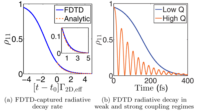
FIG. 7. (a) Population \rho_{11} dynamics within an L5 low Q -factor ( \approx 400 ) cavity, solved by MBE without any decay terms, so all phenomenological decay parameters are set to zero and the radiative decay is captured self-consistently through the local electric field used in the OBE solver. The OBEs are given initial conditions \rho_{11}(t=0) = 0.95 , \rho_{01}^{\text{lm}}(t=0) = 0 , and \rho_{01}^{\text{re}}(t=0) = \sqrt{1 - 0.95^2}/2 , such that the Bloch vector magnitude is set to unity (e.g., \sigma_1 = 2\rho_{11} - 1 , \sigma_2 = 2\rho_{01}^{\text{re}} , and \sigma_3 = 2\rho_{01}^{\text{lm}} are the usual Bloch vector components with magnitude \sigma_1^2 + \sigma_2^2 + \sigma_3^2 = 1 ). The analytic solution is determined by \Gamma_{2D, \text{eff}} , calculated by the QNM GF seen in Fig. 6(b). (b) Comparison of high- and low- Q cavities for the 2D L5 cavity structure, which were 47 000 and 430, respectively. All other parameters are the same as in (a).
