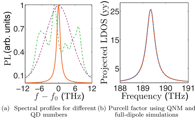
FIG. 6. (a) Modeled QD ensemble (dashed and dotted-dashed lines) for 10 (green chain) and 10 000 (magenta dashed line) QDs, for typical room-temperature inhomogeneous broadening. The individual QD line shape is given by the orange (light) line, with \gamma' = 1.5 THz. The y-shows a normalized photoluminescence (PL) for individual (solid line) and ensembled (dashed or dotted-dashed lines) QDs. The number of QDs in each simulation is on the order of 10 000. (b) Fundamental mode comparison between full-dipole expansion (blue line) and QNM theory (orange dashed line) for low- Q cavity, with a reduced PC membrane. The projected LDOS has been normalized to represent PF.
