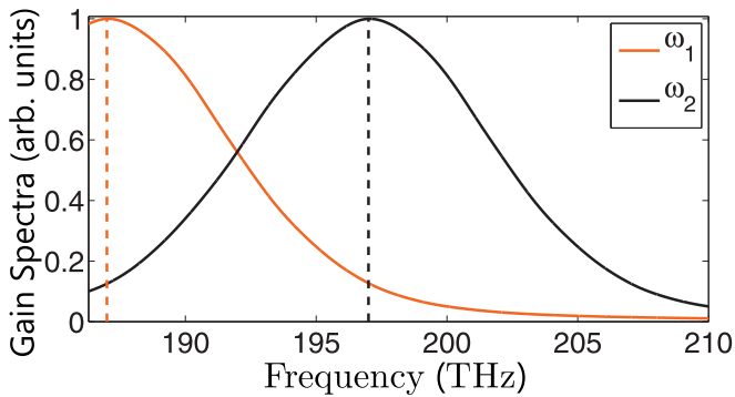
(b) Example gain profiles from QD ensemble
