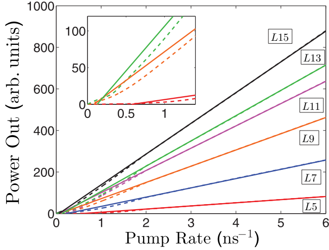
FIG. 10. Example lasing curve, or LL graphs of the \omega_1 QD ensemble, where the dashed lines represent simulated data, and solid lines are the linear fit used to extract pump threshold. The inset is a closeup of the L5 , L9 , and L13 curves.
