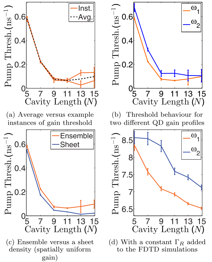
FIG. 12. Pump gain thresholds extracted from LL curves for various setups. Error bars on individual instances are determined by the maximum and minimum fitted slopes, and any uncertainty in the y intercept due to artificial power measurements at low pump strengths caused by early terminations of the simulations (as demonstrated in Fig. 13). (a) The average (dotted black line) of only two QD instances (orange lines) of \omega_1 . (b) A comparison of \omega_1 (gain model A) and \omega_2 (gain model B) simulations. (c) A comparison of the sheet simulation to the average QD simulations. (d) Thresholds given by simulations with a phenomenological radiative decay rate \Gamma_R , set to 0.05 \text{ THz} , for all QDs, for both \omega_1 and \omega_2 gain models.
