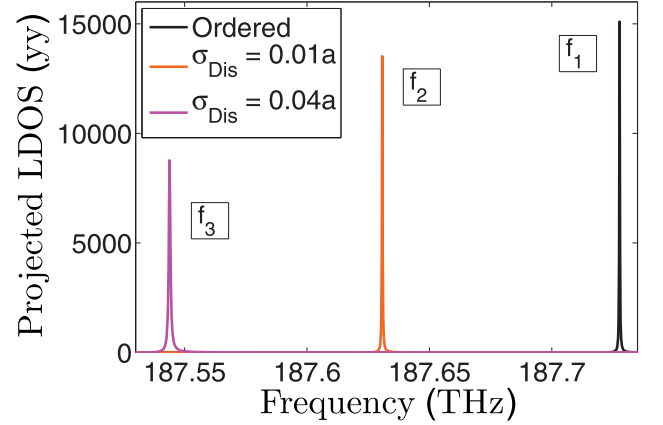
(a) L15 cavity LDOS for ordered, and disordered M1 modes
