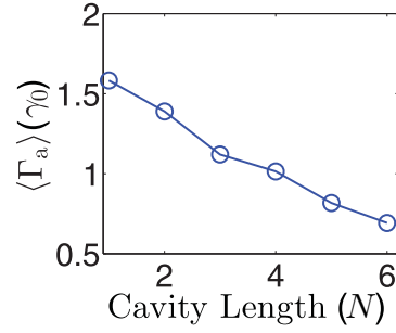
FIG. 15. Total ensemble average of the single QD radiative decay rate for each LN cavity averaged over 50 statistical variations of each instance shown in Fig. 14. In contrast to the peak Purcell factor trends, we clearly see a decrease in the average radiative decay rate for increasing cavity lengths that would be randomly sampled by the QDs.
