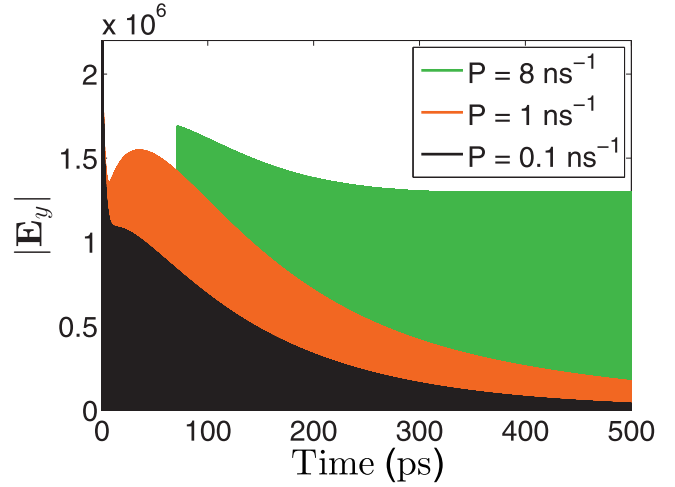
FIG. 9. Lasing dynamics (field in arbitrary units) of an L5 cavity given a QD ensemble with \omega_1 (gain model A), as measured at the center of the cavity ( x = y = 0 ). The pump rate of 0.1 \text{ ns}^{-1} does not lase and only decays, while a pump rate 1 \text{ ns}^{-1} is into the lasing regime, as it increases in amplitude, followed by decay as it finds its equilibrium, and a pump rate 8 \text{ ns}^{-1} is clearly well into the lasing regime.
