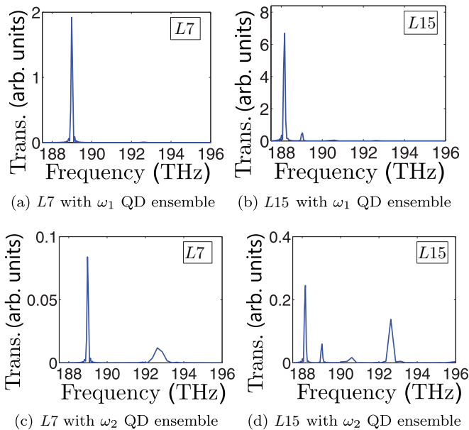
FIG. 11. (a), (b) Example transmission measured at the output power DFT monitor for lasing L7 (a) and L15 (b) cavities ( P = 8 \text{ ns}^{-1} ) the \omega_1 QD ensemble. (c), (d) Example transmission measured with the \omega_2 QD ensemble.
