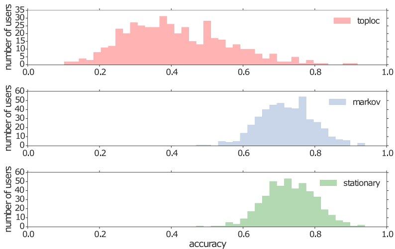
Fig 5. Accuracy of the prediction in the next-cell formulation. The top panel shows the results of the toplec strategy, that is predicting the most common location at each step. The middle panel shows the accuracy for the Markov chain model. The bottom panel shows the accuracy for the stationary strategy, that is predicting remaining in the previous cell.
