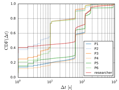
Figure 1: Cumulative Distribution Function for the time between samples \Delta t . Around 60% of the intervals of time between samples are under 10 seconds, 80% are under 60 sec, and 90% are under 200 seconds.
