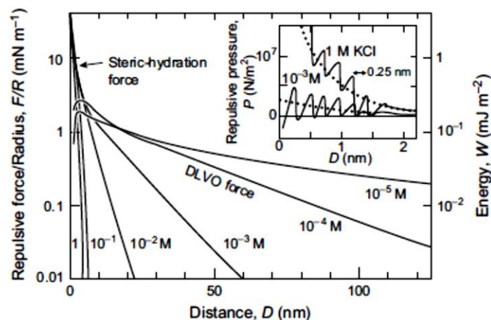
Figure 2.33 Forces between mica surfaces in 1:1 salt solutions. The right-hand axis gives the theoretical interaction energy between two flat surfaces from the Derjaguin approximation. For low salt concentrations, the theoretical DLVO theory works, while at high concentrations an additional short-ranged hydration repulsion is produced due to the presence of adsorbed cations.[220]
