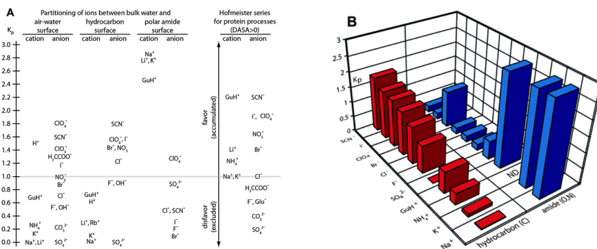
Figure 2.28 Partition coefficients for the cations and anions at nonpolar and polar surfaces.[199]
