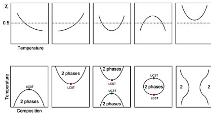
Figure 2.9 Different types of polymer solution phase diagrams resulting from temperature-dependence of the Flory Huggins interaction parameter.[20]
