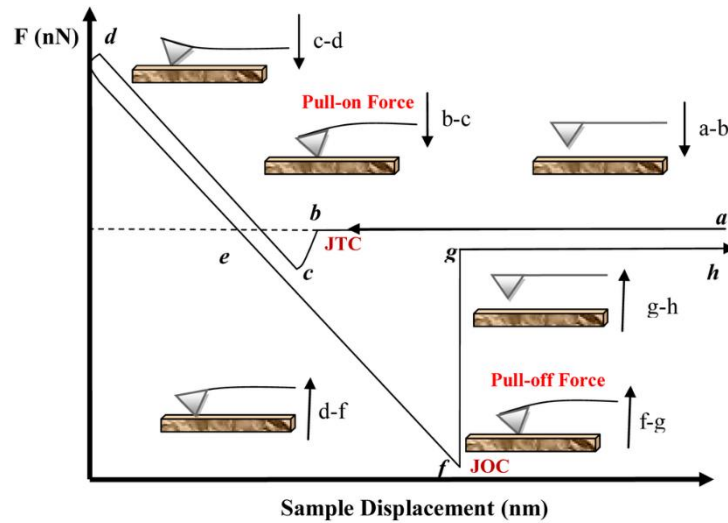
Figure 3.12 Typical AFM force-distance profile.[287] (a-b) at far separation distance where no interaction between the probe and surface is found. (b-c) close to the surface, an attractive interaction causes jump-in . (c-d) the cantilever is pressed on the surface. (d-f) the cantilever is retracted from the surface. (f-g) the tip leaves the surface. (g-h) far separations where no interaction is found. This procedure provides the force-distance profile at one point of surface. To obtain statistically reliable data, the force measurements are performed on various points over a surface area.
