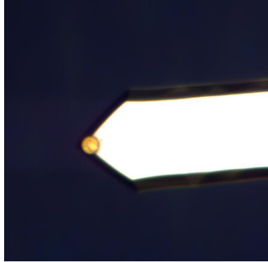
Figure 3.11 7 \mu\text{m} silica particle attached to the tipless cantilever using the described method.
