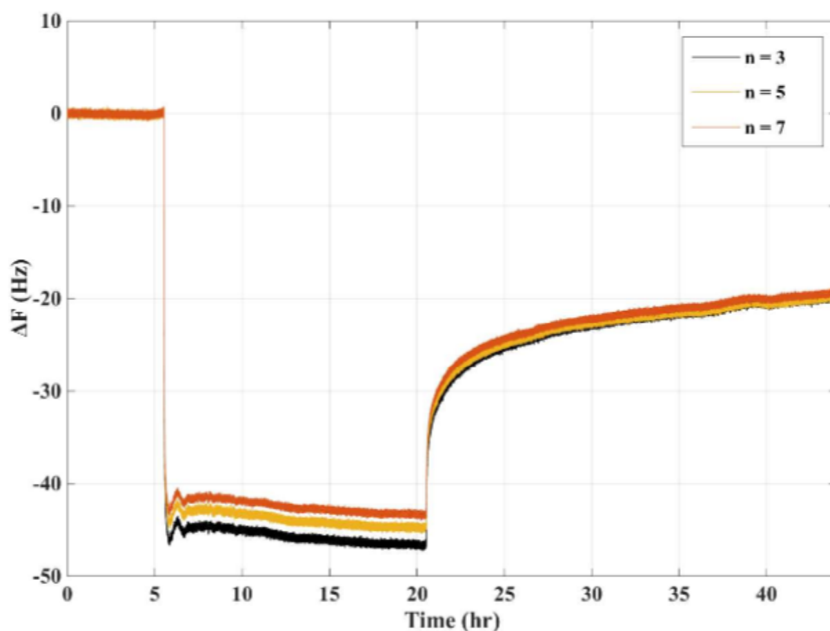
Fig. S2 Frequency shift resulting from adsorption of the thiol-terminated PNIPAM (0.1 wt% solution) on the gold sensor;
