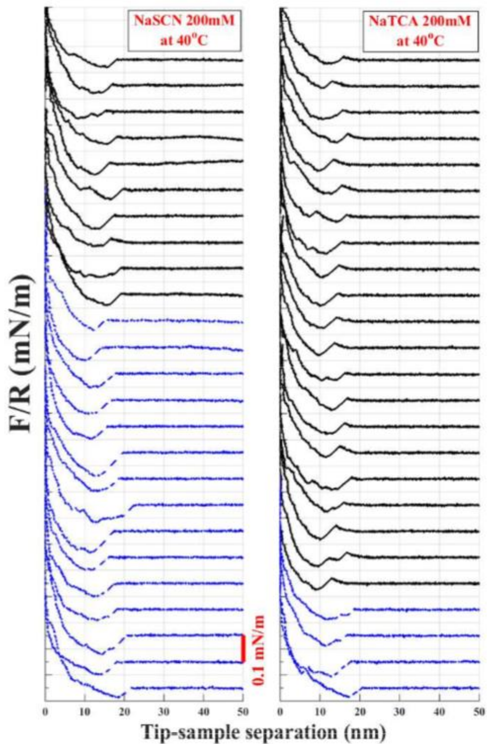
Fig. S13 Approach force-distance curves between the PNIPAM layers in NaSCN 200mM and NaTCA 200mM at 40 °C. Black full lines represent measurements where a weak repulsion was observed before jump-in the surface. As shown, 21 out of 25 curves in NaTCA show initial repulsion, while it is 10 out of 25 curves in NaSCN.
