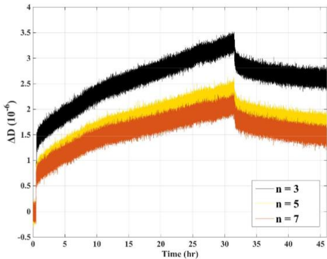
Fig. S6 Dissipation shift resulting from physical adsorption of PNIPAM on the gold sensor; the positive shift in dissipation indicates formation of a viscoelastic polymer film on the sensor. The overtone-dependence of the dissipation shift further confirms viscoelasticity of the formed layer. Rinsing with water leads to a decrement in the dissipation factor, which can be assigned to desorption of the weakly attached PNIPAM chains.
