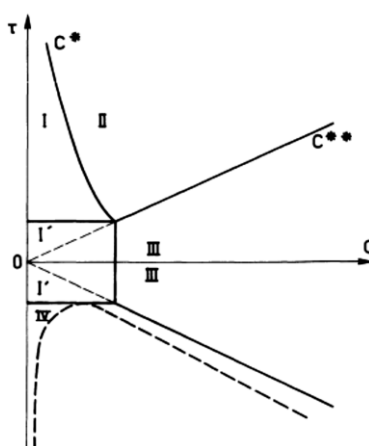
Figure 2.10 Typical phase diagram of a polymer solution, suggested by Daoud and Jannink. \tau is the reduced temperature defined as \frac{T-\theta}{\theta} . [21]
