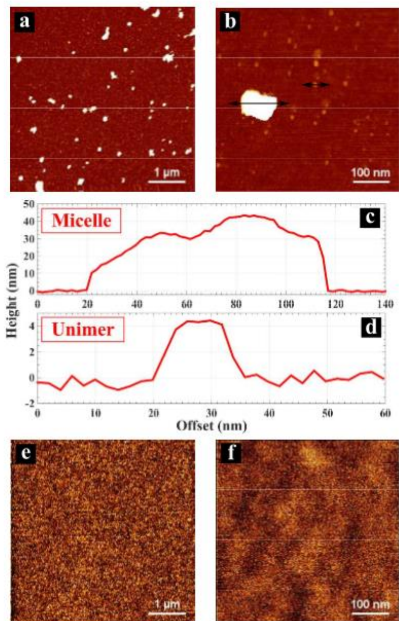
Figure 3 Topography of the copolymers on the silica surface at 20 °C; (a)(b) Height images of PNIPAM-PAMPTMA diblock (c)(d) cross-section profiles of a micelle and a unimer, which are indicated on figure b. (e)(f) Height images of MPEG-PNIPAM-PAMPTMA triblock
