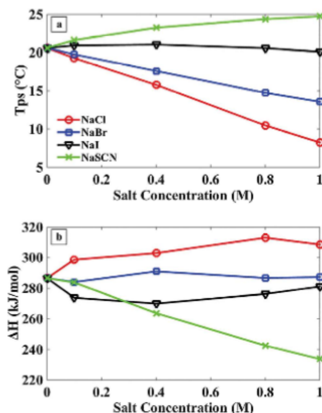
Fig. 2 DSC data of 0.5 wt% PPO in different salts solutions. (a) Phase separation temperature and (b) enthalpy change of dehydration.
