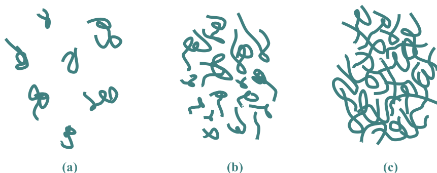
Figure 2.11 Polymer solution concentration regimes: (a) Separated chains, (b) Overlapping chains, (c) Overlapping comparable to bulk polymer state.
