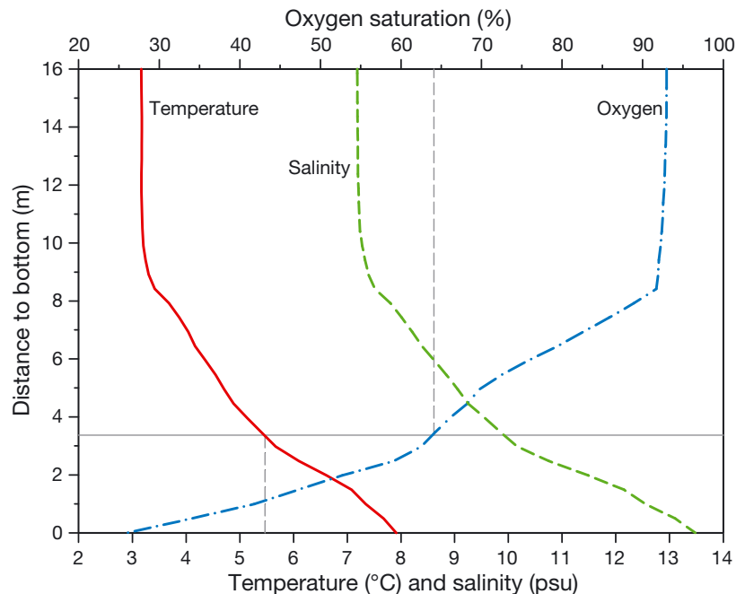
Fig. 2. Generalized vertical profiles of temperature, salinity and oxygen saturation in the lower part of the ~64 m water column obtained from 9 CTD stations (conditions are constant above this part of the water column). Horizontal line: mean of the daytime vertical distribution of Atlantic cod Gadus morhua (detected single target echoes of strengths between -30 and -24 dB); dashed lines: corresponding temperature and oxygen saturation of the water
