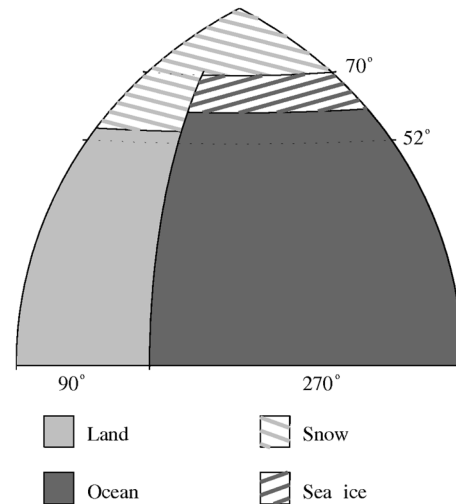
Figure 2. Model configuration. The model consists of one hemisphere divided by 52° latitude into 360° wide, low–mid-latitude (LL) and high-latitude (HL) sectors. Values for global reservoirs, transports and fluxes are twice the hemispheric values. The model ocean is 270° wide and extends from the Equator to 70° latitude. The ocean covers 70.5 % of the model surface. LL and HL ocean sectors have the area ratio 84 : 16. Sea ice and snow coverage are diagnosed from idealized, meridional profiles of atmospheric temperature.
