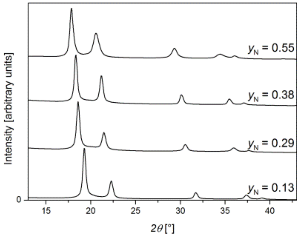
Fig. 1. X-ray diffractograms of 12.5 μm AISI 316 foils annealed at 1323 K and nitrated in NH 3 /H 2 gas mixtures at 693 K. Nitriding potentials less than infinity were applied after full saturation was achieved. Increasing nitrogen content causes increasing shifts of reflections towards lower diffraction angle ( 2\theta ).
