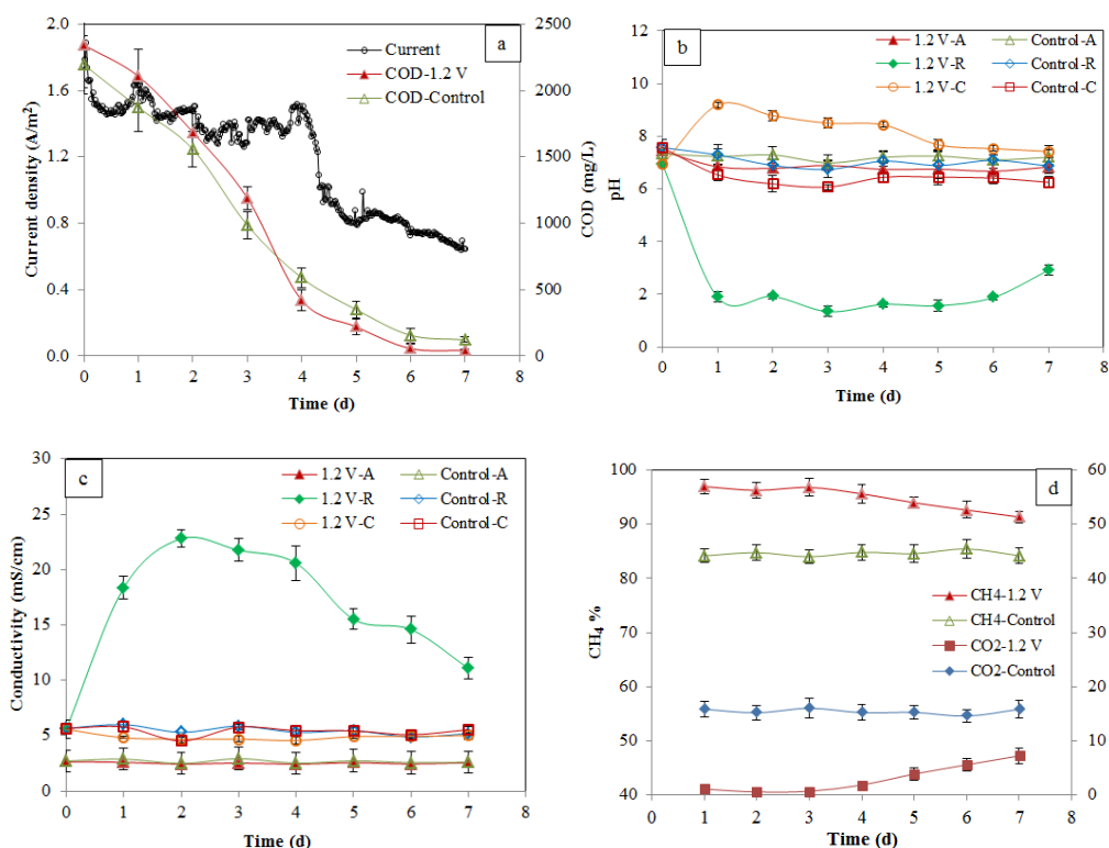
Figure 9. MESC performance at 19.6 mL/h gas flow rate with 1.2 V and control experiment. A, anode chamber; R, regeneration chamber; C, cathode chamber. The current density output and COD changes (a); pH profiles in three chambers (b); conductivity profiles in three chambers (c); methane and carbon dioxide contents in the outlet gas (d). ( Paper III )
