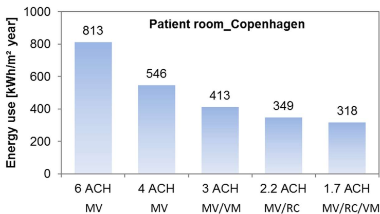
Figure 36: Annual energy use for the air-conditioning systems in a double patient room in Copenhagen.
