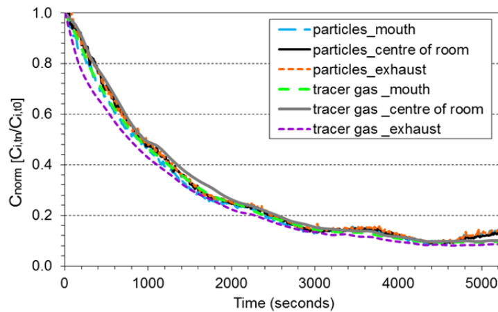
Figure 5. Comparison of the normalized 0.7 \mu\text{m} particle concentration with tracer gas normalized concentration based on release close to the manikin's body, and effect of local exhaust ventilation.
