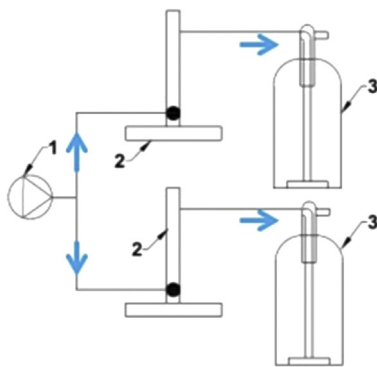
Fig. 5. Diagrammatic representation of the NH 3 gas generation setup, where 1 – pump, 2 – gas Rotameter and 3 – washing bottle with NH 4 OH solution.
