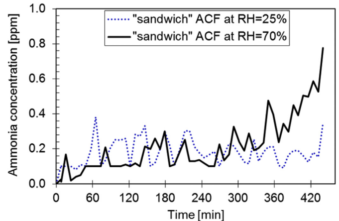
Fig. 10. Ammonia gas concentration measured in the exhaust duct of the VM downstream of the "sandwich" ACF material in the cases the relative humidity was 25% and 70% in the room.
