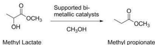
Scheme 1. HDO of ML to MP in methanol
