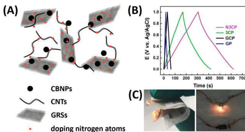
Fig.1 (A) Schematic for the heterostructure of the prepared nitrogen-doped multi-dimensional carbon materials. (B) Charge-discharge curves of different paper electrodes at 1 A·g -1 . (C) A lab-made N3CP based flexible supercapacitor (left) and a miniature bulb is lightened up by such a flexible supercapacitor (right). Not drawn to scale.
