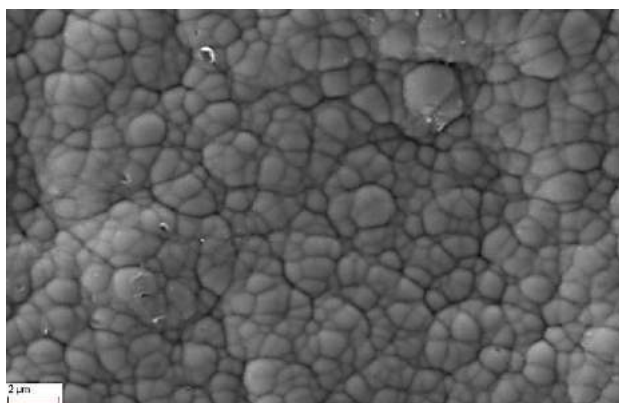
Figure 1. SEM image of the surface of cathodes covered with LiPON thin films (1µm)
