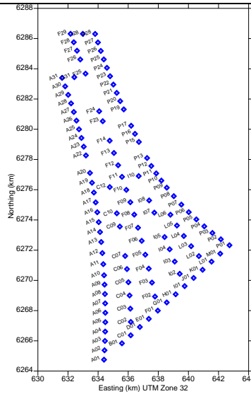
Figure 5. The Anholt wind farm layout
