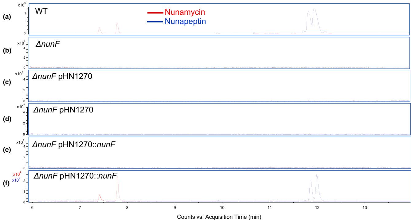
FIGURE 6 Liquid chromatography–high-resolution mass spectrometry (LC-HRMS) analysis of Pseudomonas fluorescens In5 WT, \Delta nunF , and complemented mutant. Strains of P. fluorescens In5 WT (a), \Delta nunF (b), \Delta nunF pHN1270 0 mmol/L IPTG (c), \Delta nunF pHN1270 2 mmol/L IPTG (d), \Delta nunF pHN1270:: nunF 0 mmol/L IPTG (e), and \Delta nunF pHN1270:: nunF 2 mmol/L IPTG (f) were grown on fifth strength PDA for 48 hr at 20°C. Peptide extraction was performed on agar and biomass using 2-butanol containing 1% formic acid followed by ultrasonication and evaporation of the organic phase under nitrogen. Samples were resuspended in methanol. LC-HRMS analysis was performed in triplicate. Extracted ion Chromatograms (EICs) of proton adducts of nunamycin (red) and nunapeptin (blue)
