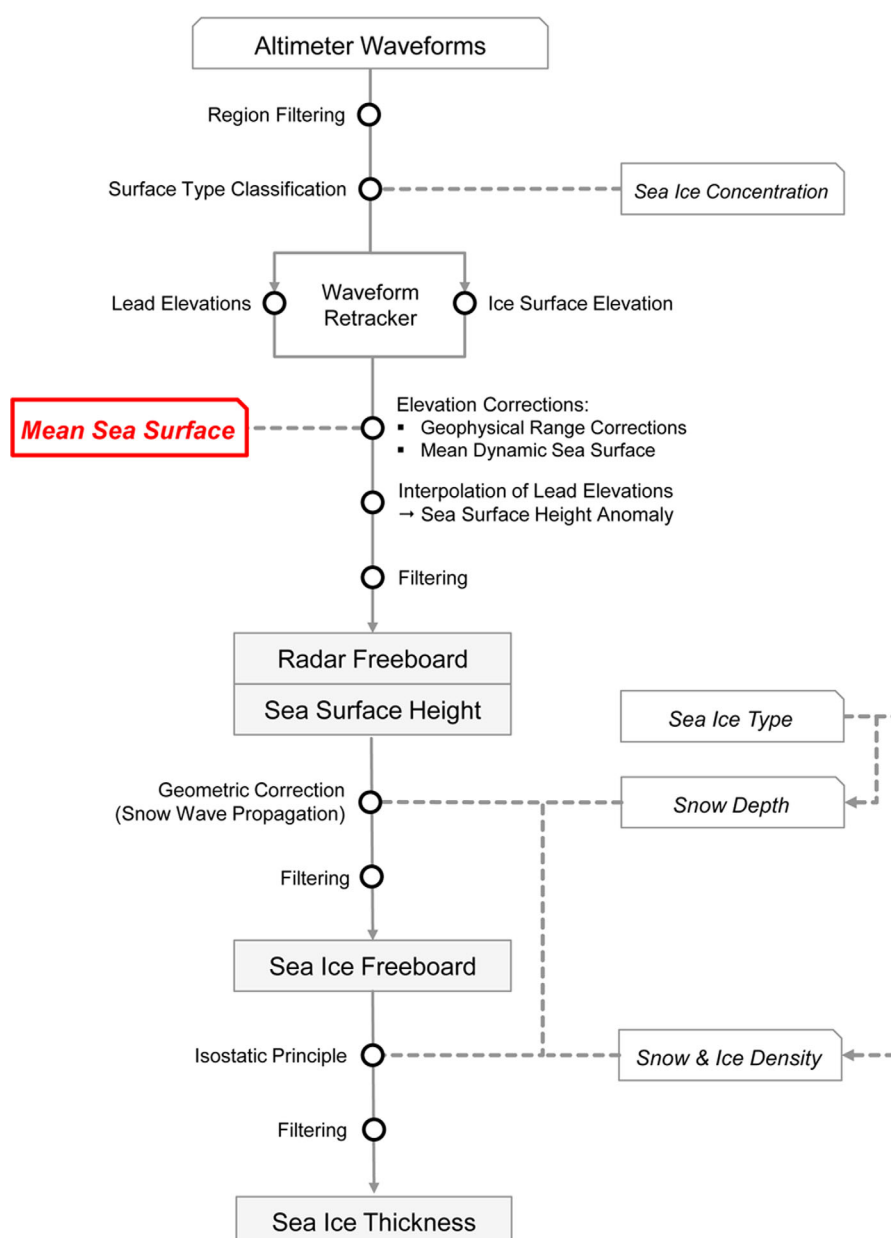
Figure 6. Example of algorithm employed at the Alfred Wegener Institute (AWI) to derive sea ice freeboard and thickness (Ricker et al., 2014). The step where the respective MSS or GGM model is subtracted, is highlighted in red, and occurs at the same point when the geophysical range corrections are applied, and before lead elevations are interpolated along-track to calculate the local sea surface height anomaly (SSHA) about the MSS/GGM.
