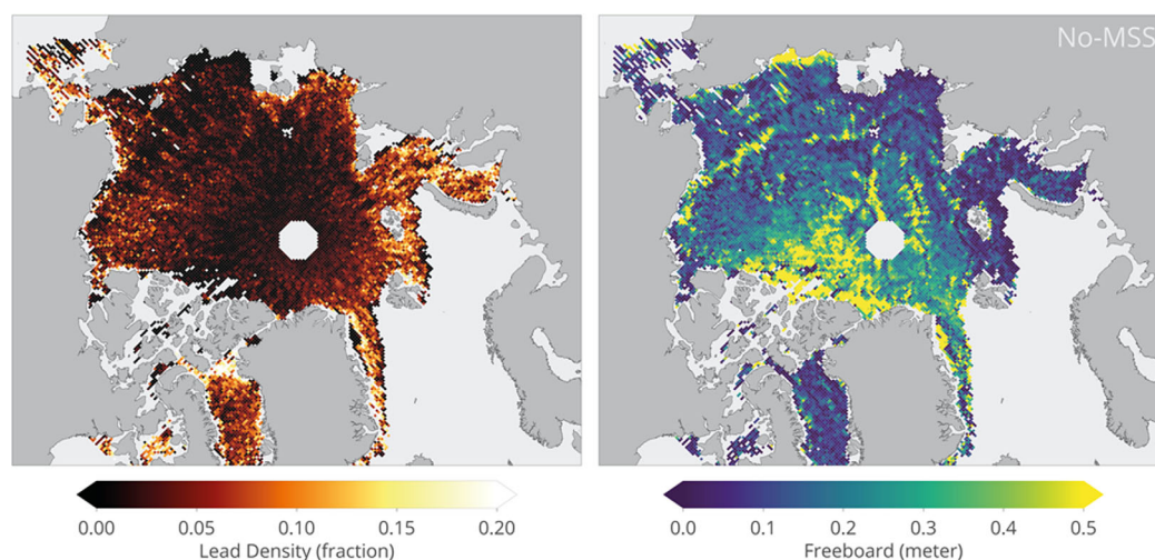
Figure 8. (left) Geographical distribution of leads for April 2015 given by the lead fraction defined as the ratio of the number of waveforms classified as lead returns to the total number of positively identified waveforms. Sea ice freeboards when no MSS/GGM field is applied in the processing chain, revealing anomalous freeboard values associated with short-wavelength gravity anomalies and steep gravity gradients.
