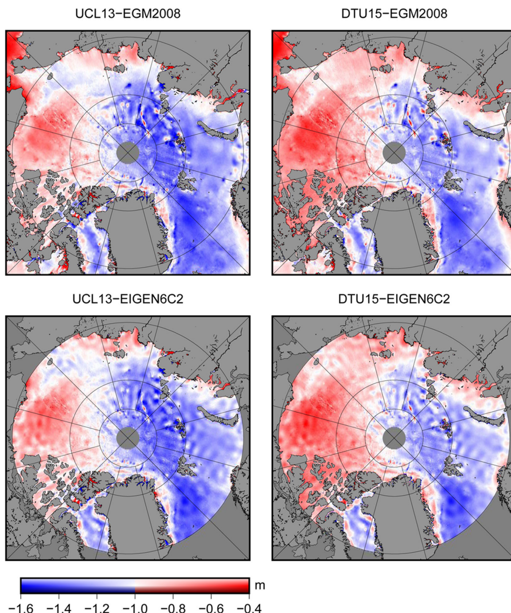
Figure 5. Comparison of mean dynamic topography (MDT) mapping in the Arctic Ocean by combining state-of-the-art UCL13 and DTU15 MSS fields with GGM EGM2008 and gravimetric geoid model EIGEN6C2.
