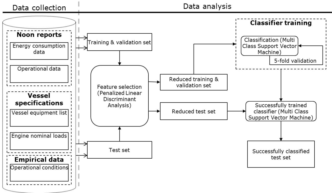
Figure 3: Flowchart of proposed algorithm
