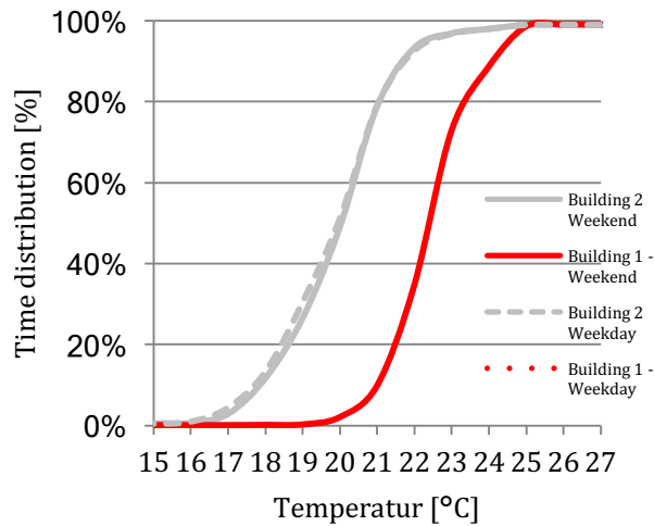
Figure 7 Average temperature summation curve for weekdays and weekends in the heating season [°C].
