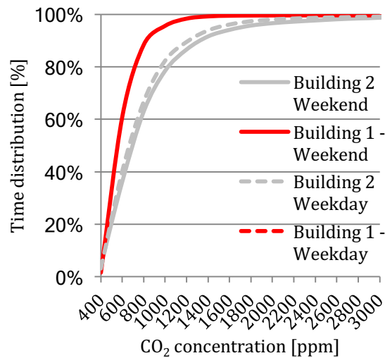
Figure 8 Average CO 2 concentration summation curve for weekdays and weekends in the heating season [ppm]
