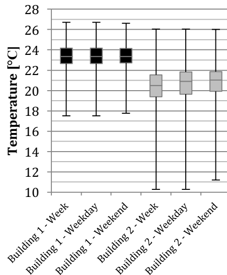
Figure 1 Boxplot representing the median, 25 th percentile, 75 th percentile and min/max measurements of the temperature [°C] from March 2013 through April 2013.
