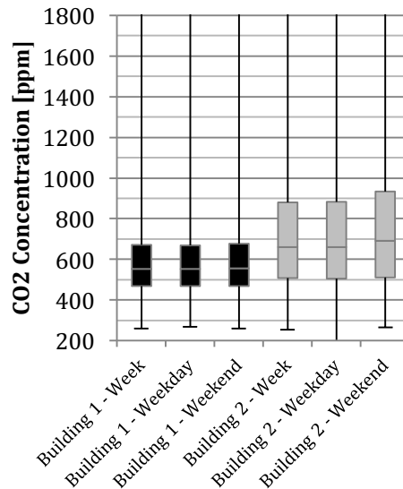
Figure 3: Boxplot representing the median, 25 th percentile, 75 th percentile and min/max measurements of the CO 2 concentration [ppm] from March 2013 through April 2013.
