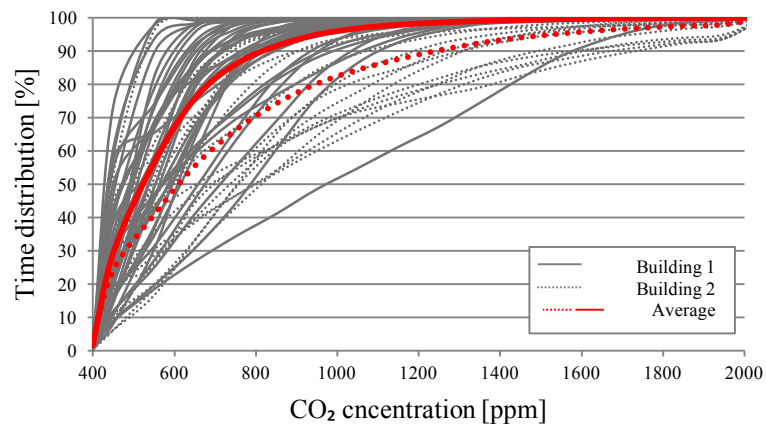
Figure 4 Average CO 2 concentration summation curve of Building 1 and Building 2, and CO 2 concentration summation curve of each apartment [ppm]
