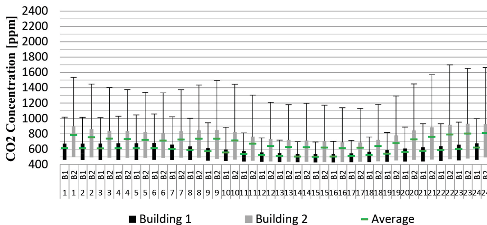
Figure 11 Hourly CO 2 concentration distribution of Building 1 (Black) and Building 2 (Grey), with the box representing the 25 th and 75 th percentile. Whisker representing the 95 th percentile. Green mark shows the average value.
