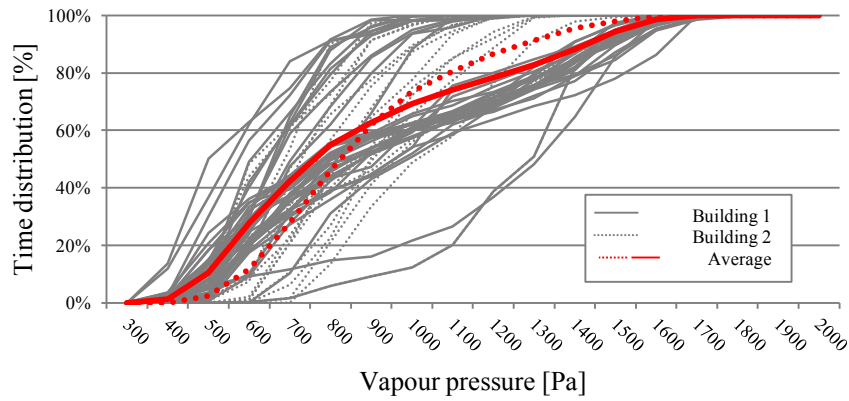
Figure 6 Average vapour pressure summation curve of Building 1 and Building 2, and vapour pressure summation curve of each apartment [Pa]
