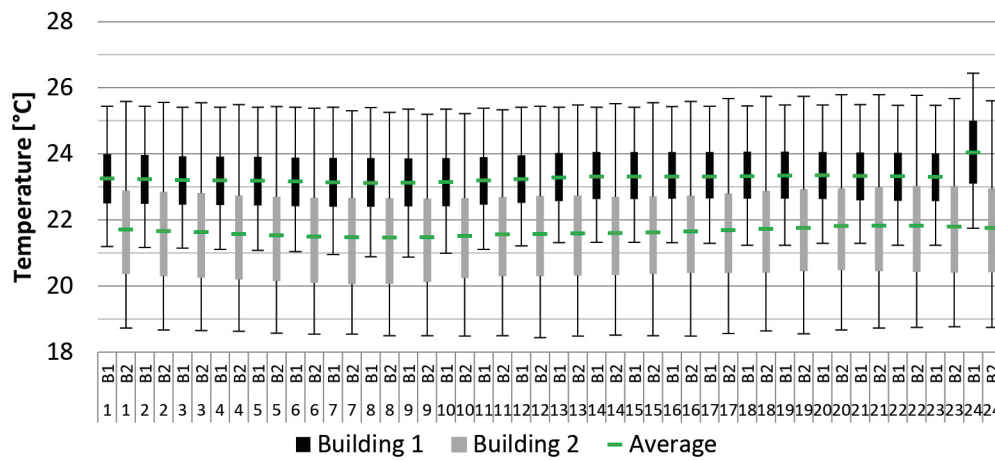
Figure 10 Hourly temperature distribution of Building 1 (Black) and Building 2 (Grey), with the box representing the 25 th and 75 th percentile. Whiskers representing the 5 th and 95 th percentile. Green mark shows the average value.
