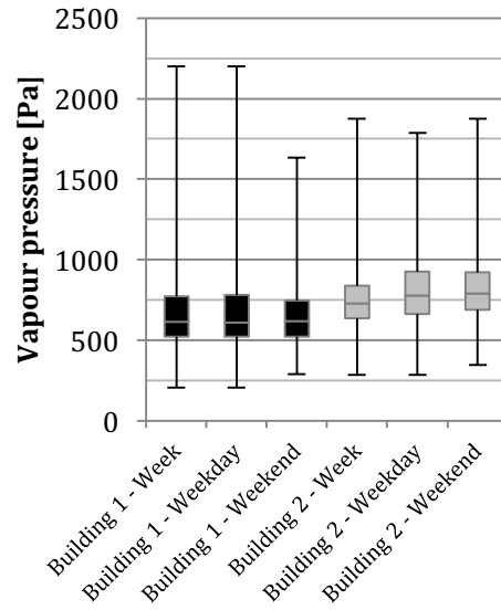
Figure 5 Boxplot representing the median, 25 th percentile, 75 th percentile and min/max measurements of the tvapour pressure [Pa] from March 2013 through April 2013.
