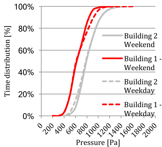
Figure 9 Average vapour pressure summation curve for weekdays and weekends in the heating season [Pa].
