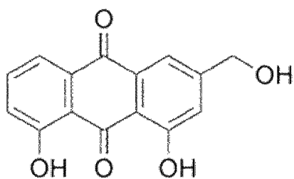
9,10-anthraquinone skeleton
