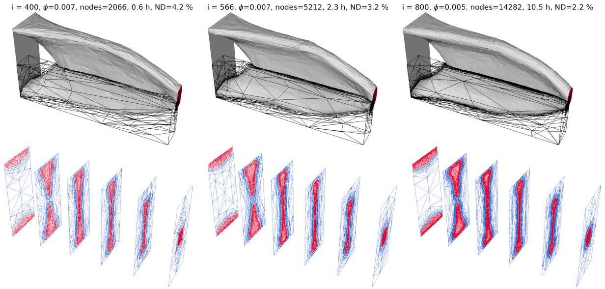
Fig. 7. The result of optimizing for a single load case is shown by means of an iso-surface and slices orthogonal to the x -direction. All optimizations give an I-beam design, but there are large variations in the objective functions. The corresponding optimization with a fixed mesh is shown in figure 9 (left).
