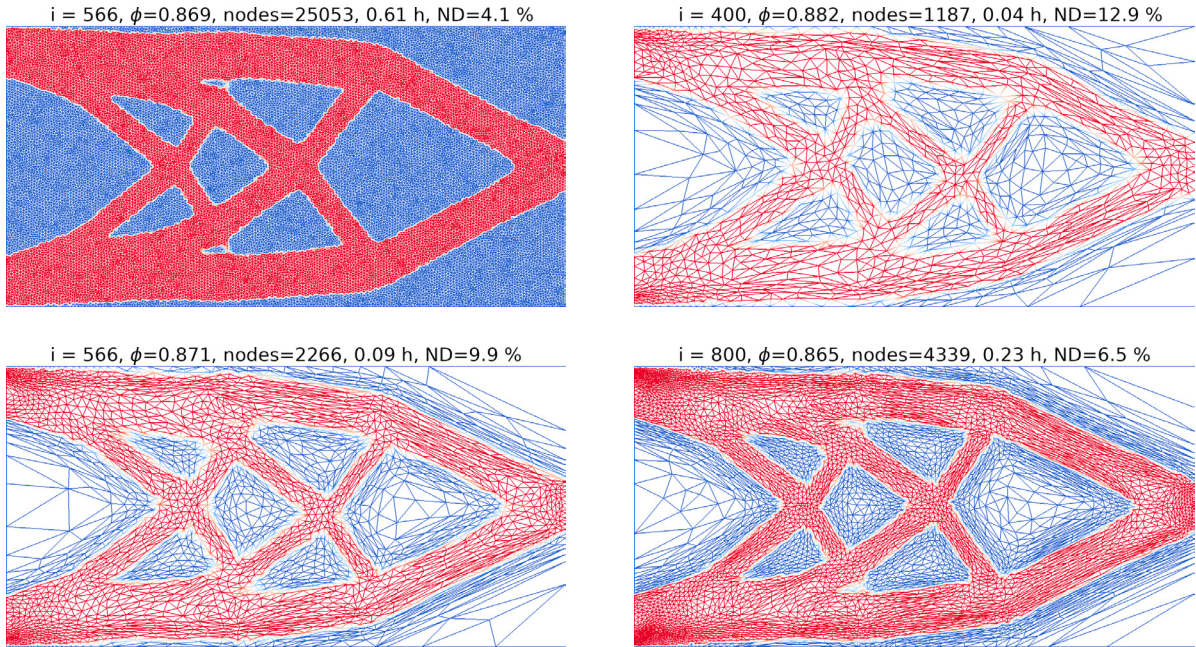
Fig. 5. The results of optimizations No 1-4 (see table 1) indicate that the dynamic meshes give rise to the same topology with less computational effort.
