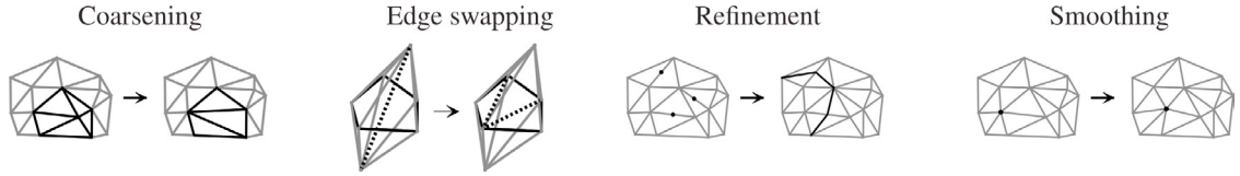
Fig. 1. Four local mesh modification operations are sketched. None of the operations are allowed to decrease worst local element quality associated with the operation, except for coarsening in 3D. The operations are implemented in the adapt_rmnd , adapt_flipedg , adapt_add_nd and adapt_mvnd functions. Note that we do not apply 3D face swapping (also called 2-to-3 swapping), because the applied implementation has been found [13] to generate equally good meshes without it.
