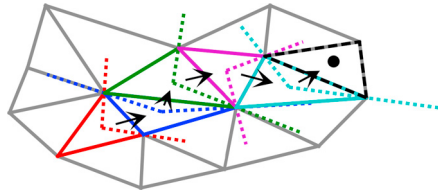
Fig. 2. The information required for interpolating a nodal field is preserved during the mesh adaptation by relying on the fact that we can guess an element (red) close to the element containing the old node. By dividing the domain in 3 (4 in 3D), we can make a decision as to which of the neighboring elements is the better candidate. We continue this process until the correct element is found (dashed black). This functionality is implemented in the elem_interp and elem_find functions.
