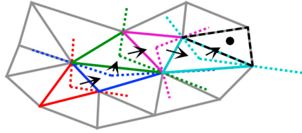
Fig. 2. The information required for interpolating a nodal field is preserved during the mesh adaptation by relying on the fact that we can guess an element (red) close to the element containing the old node. By dividing the domain in 3 (4 in 3D), we can make a decision as to which of the neighboring elements is the better candidate. We continue this process until the correct element is found (dashed black). This functionality is implemented in the elem_interp and elem_find functions.
