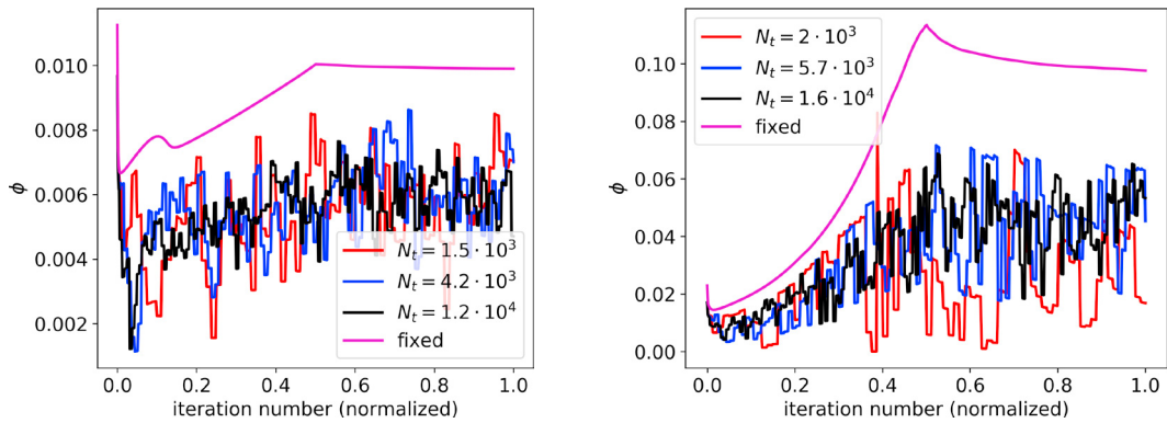
Fig. 10. The dynamic meshes give rise to large oscillations in 3D, but they still outperform the fixed meshes.
