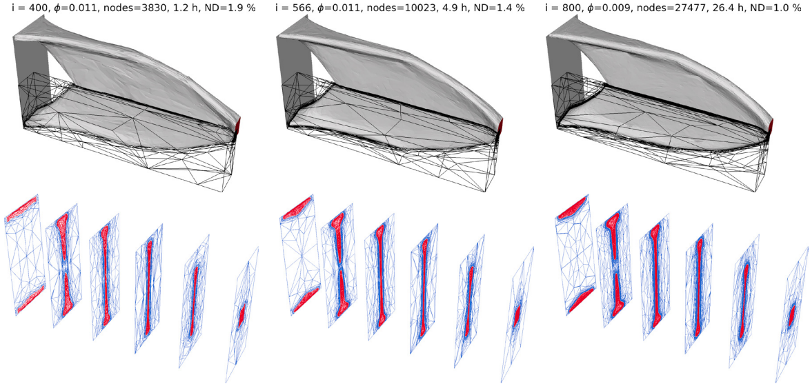
Fig. B.12. The result of optimizing for a single load case with V_{frac}=0.1 is shown. The design is topologically independent, but there is a slight variation in the gap size for slice # 2.
