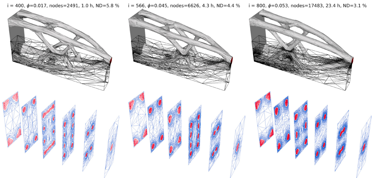
Fig. 8. Optimizing for two load cases leads to truss-structure, which appears to be mesh independent, but there are some variation in slice 3, 4 and 5, which we attribute to minor differences between the designs. Figure 9(right) shows the corresponding optimization with a fixed mesh.
