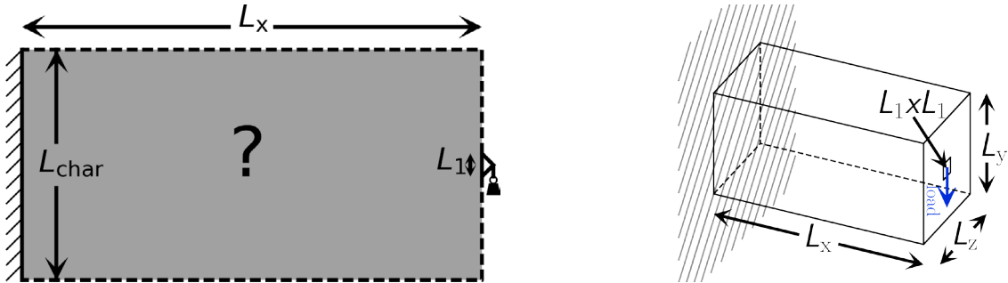
Fig. 4. The 2D and 3D cantilever problems are plotted with the support to the left and the load to the right. The initial volume and boundary mesh for these problems are generated in the mesh_cant and mesh_cant3D functions.
