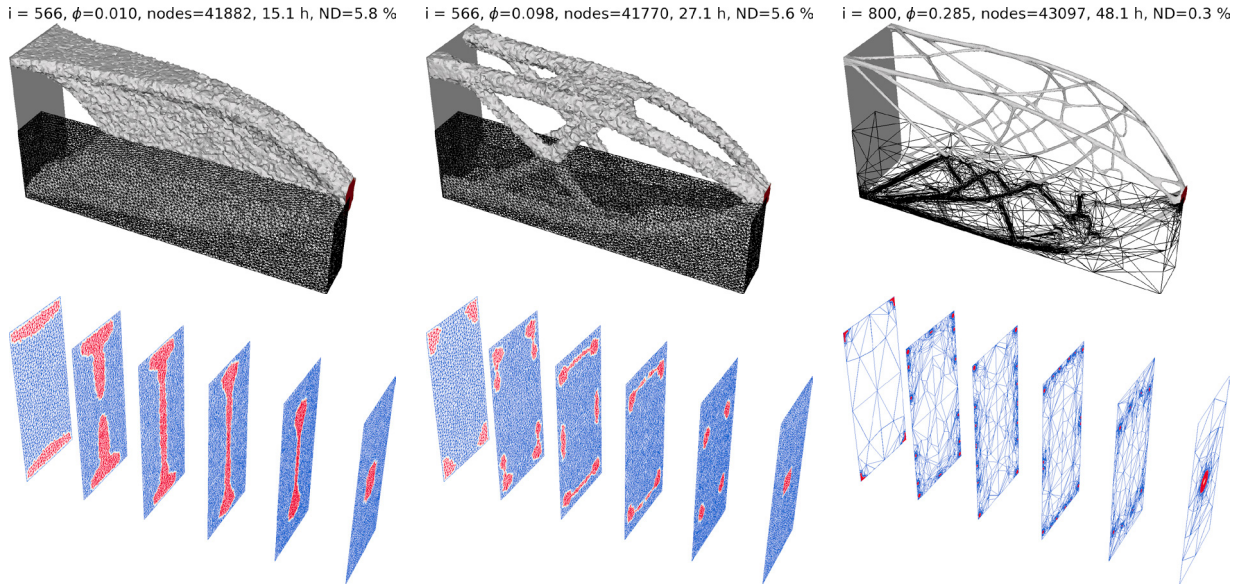
Fig. 9. The results of the 3D optimizations with fixed meshes (No 5 and 9) are shown for one (left) and two load cases (center). The corresponding optimization with fixed meshes are shown in figures 7 and 8. Note that the large linear systems associated with these optimizations require significant amounts of memory. Finally, the result of optimization No 13 is shown to the right.
