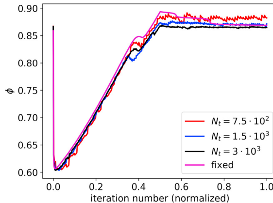
Fig. 6. The objective functions for the 2D optimizations are plotted versus the normalized iteration number. The dynamic meshes tend to produce some oscillations, particularly for the coarse meshes, but the dynamic meshes consistently gives better objective functions than the fixed mesh.
