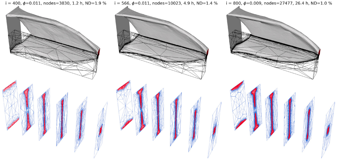
Fig. B.12. The result of optimizing for a single load case with V_{\text{frac}}=0.1 is shown. The design is topologically independent, but there is a slight variation in the gap size for slice # 2.
