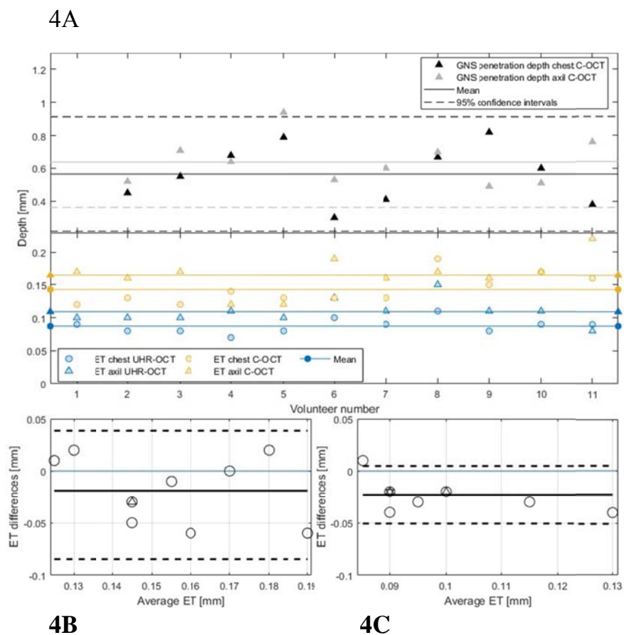
Figure 4: Epidermal thickness and penetration depth of gold nanoshells in OCT images from armpit and chest
