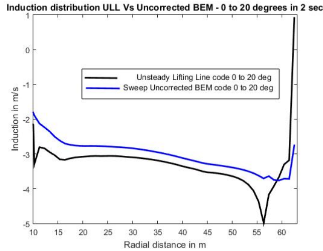
Fig. 7 Comparative diagram of induction distribution for the 10% tip aft swept at 20 degrees NREL 5MW rotor predicted by ULL and BEM.
