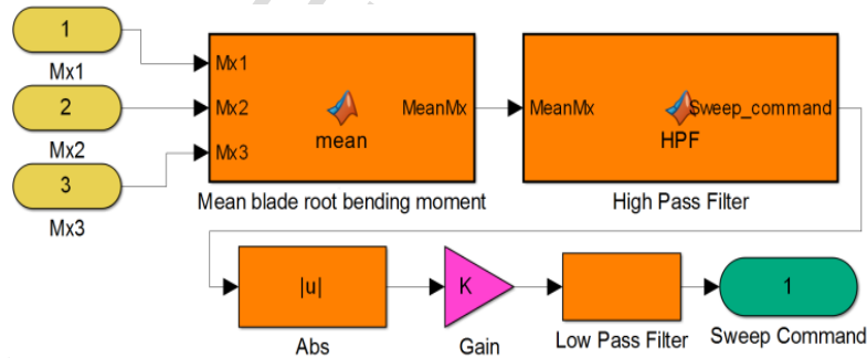
Fig. 13 The control method for load reduction in Matlab Simulink - M_{x1} , M_{x2} , M_{x3} are the root bending moments of the 3 blades
