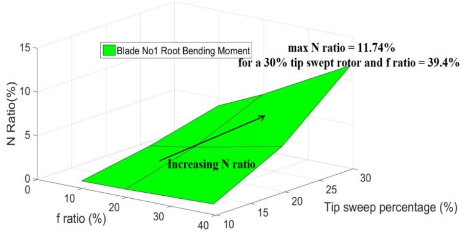
Fig. 12 Nratio vs fratio for Blade No1 root bending moment concerning a 10%, 20%, 30% tip swept rotor at rated operation ( V=11.4\text{m/s} ) and sweep angle variation according to \Lambda=10\sin(\omega t) for \omega = \pi/4, \pi/2, \pi
