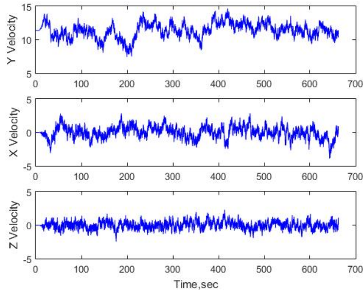
Fig. 16 The three wind velocity components at hub height for the examined test case
