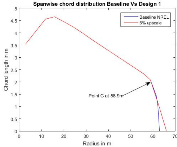
Fig. 14 NREL Vs New Blade design chord length distribution
