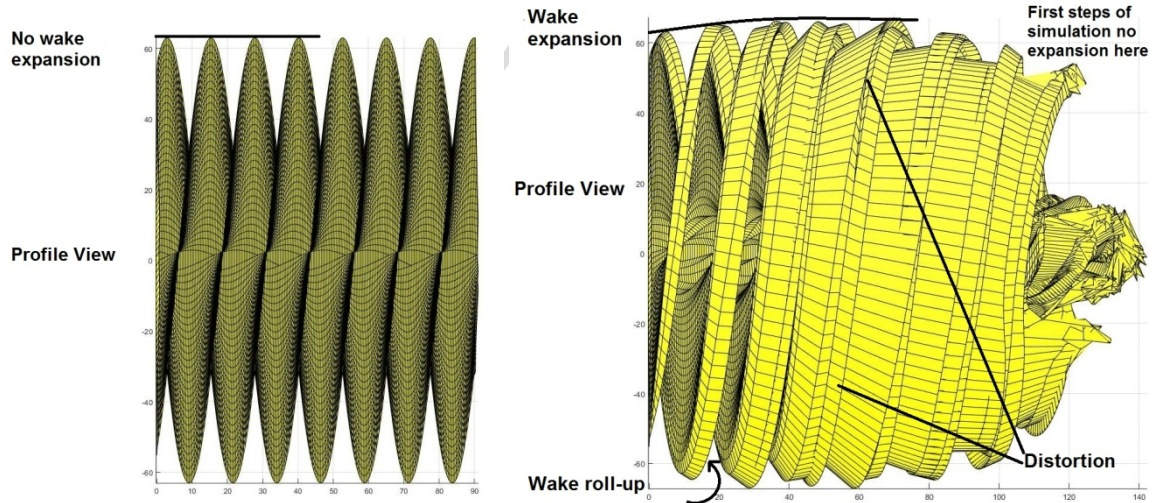
Fig. 4 : Prescribed wake development versus free wake development behind a 5MW NREL wind turbine rotor – profile view
