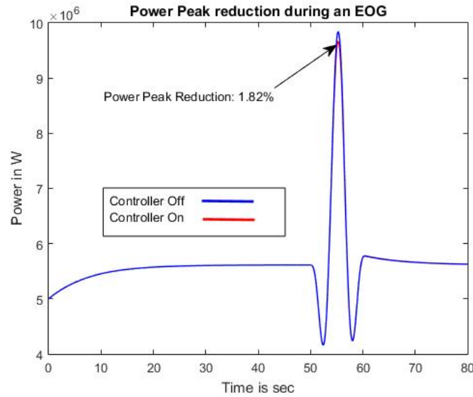
Fig. 22 Wind Turbine Power Peak reduction during an EOG for 10% tip swept rotor.
