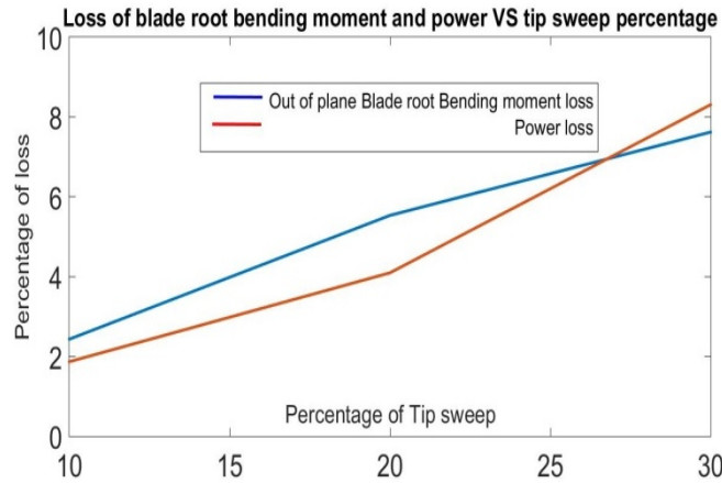
Fig. 23 Extreme load reduction and power peak reduction percentages in relation to rotor tip sweep percentage of 5MW NREL wind turbine.
