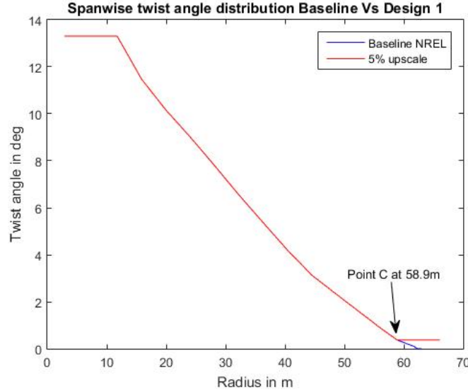
Fig. 15 NREL Vs New Blade design twist angle distribution
