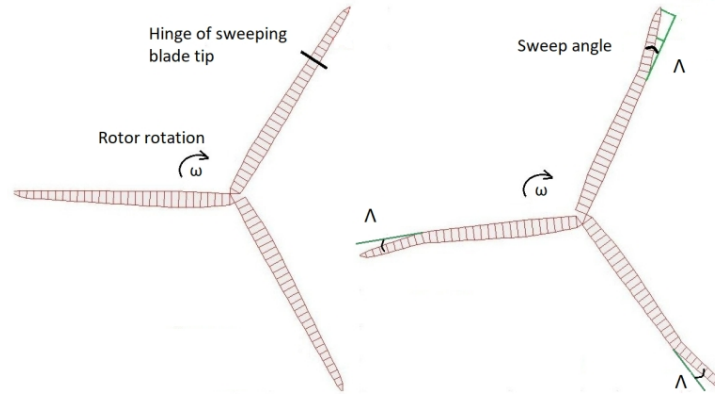
Fig. 1 Wind Turbine Rotor sweeping aft to compensate for a wind gust – Left: Sweep Angle \Lambda=0 , Right: Sweep Angle \Lambda in aft position
