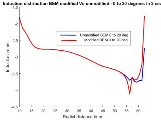
Fig. 9 Induction distribution curves for sweep modified and unmodified BEM code 20 deg aft sweep 10% tip sweep
