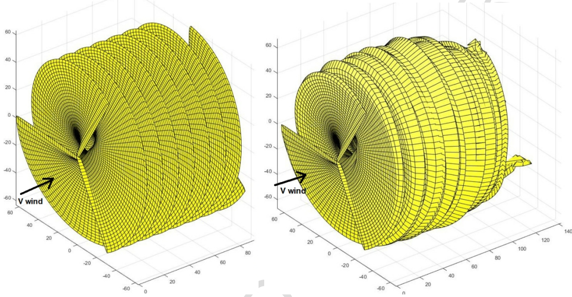
Fig. 3 : Prescribed wake development versus free wake development behind a 5MW NREL wind turbine rotor
