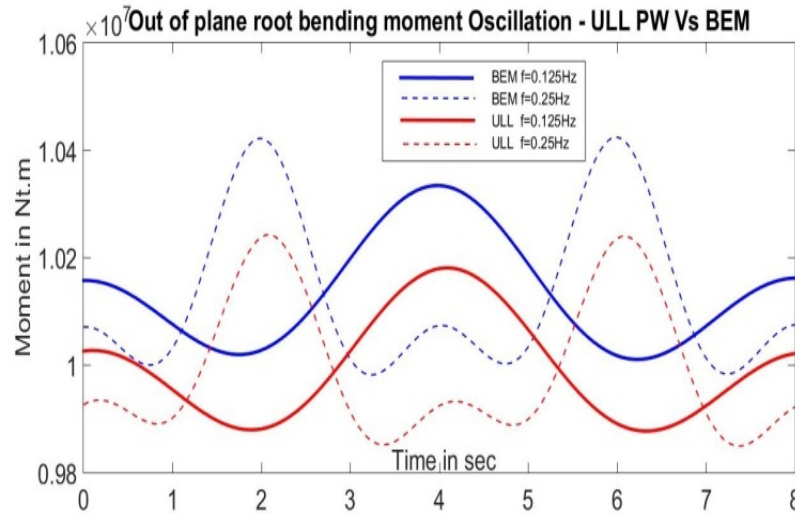
Fig. 6 Comparative diagram of Blade 1 root bending moment oscillation for the 20% tip swept NREL 5MW rotor predicted by ULL and BEM. Amplitude = 12deg - frequency = 0.125 and 0.25Hz - t=0 tip starts with aft sweep.
