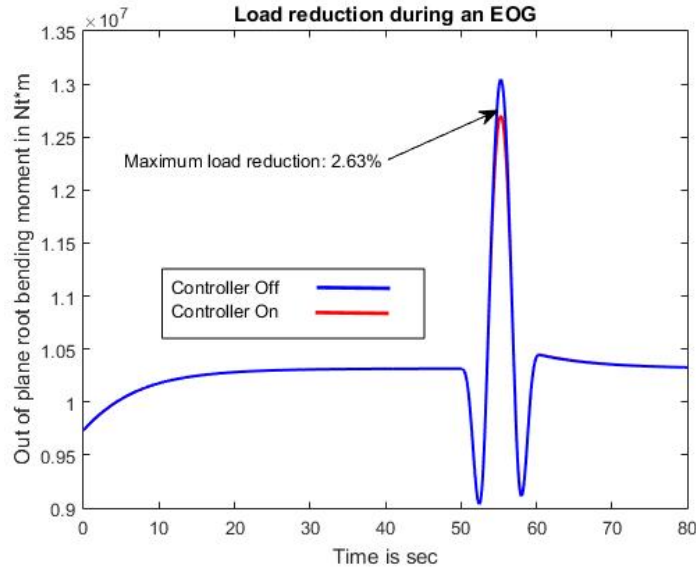
Fig. 21 Out of plane root bending moment of Blade No1 during an EOG for 10% tip swept rotor.
