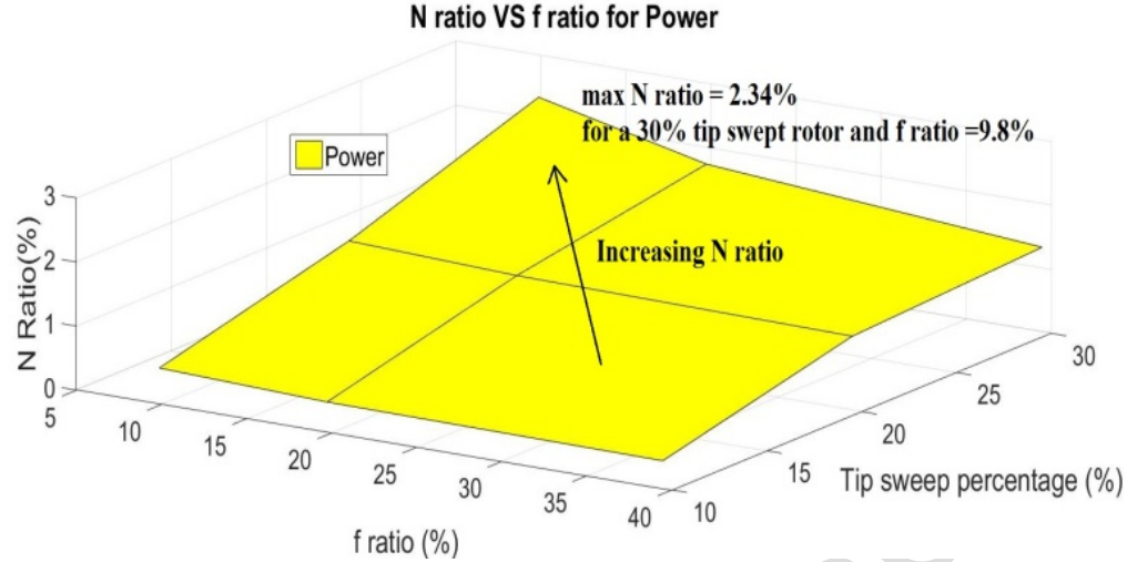
Fig. 11 Nratio vs fratio for Power concerning a 10%, 20%, 30% tip swept rotor at rated operation ( V=11.4\text{m/s} ) and sweep angle variation according to \Lambda=10\sin(\omega t) for \omega = \pi/4, \pi/2, \pi
