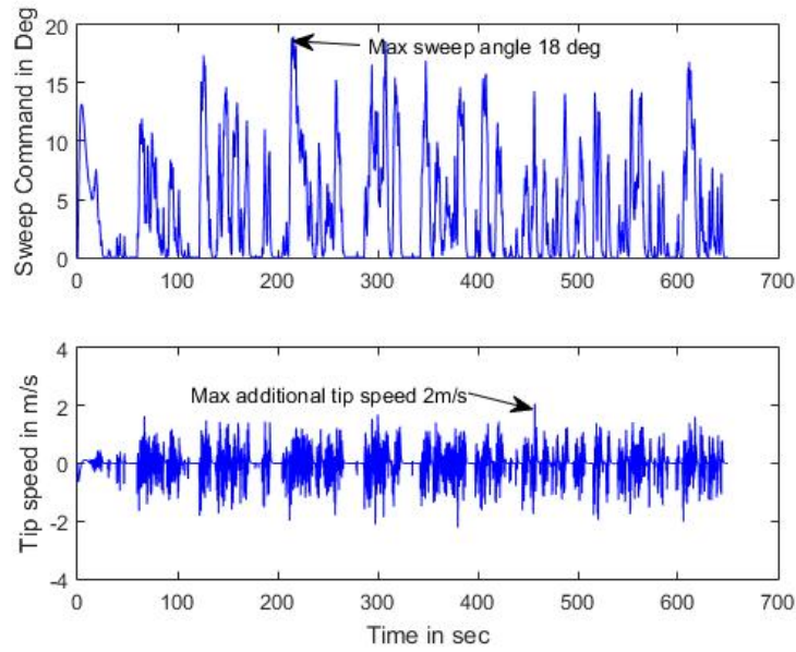
Fig. 17 Tip sweep angle response during a turbulent wind input for the modified NREL wind turbine.
