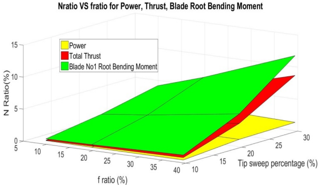
Fig. 10 Nratio vs fratio for Power Total thrust and Blade No1 root bending moment concerning a 10%, 20%, 30% tip swept rotor at rated operation ( V=11.4\text{m/s} ) and sweep angle variation according to \Lambda=10\sin(\omega t) for \omega = \pi/4, \pi/2, \pi
