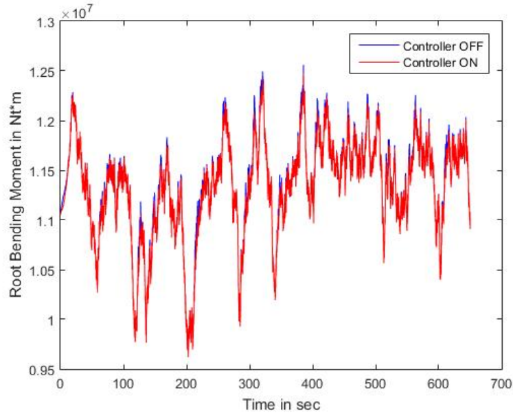
Fig. 18 Fatigue load reduction during a turbulent wind input for the modified NREL wind turbine.
