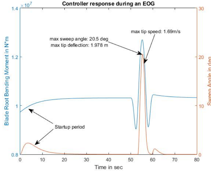
Fig. 20 Tip sweep angle response during an EOG for 10% tip swept rotor.
