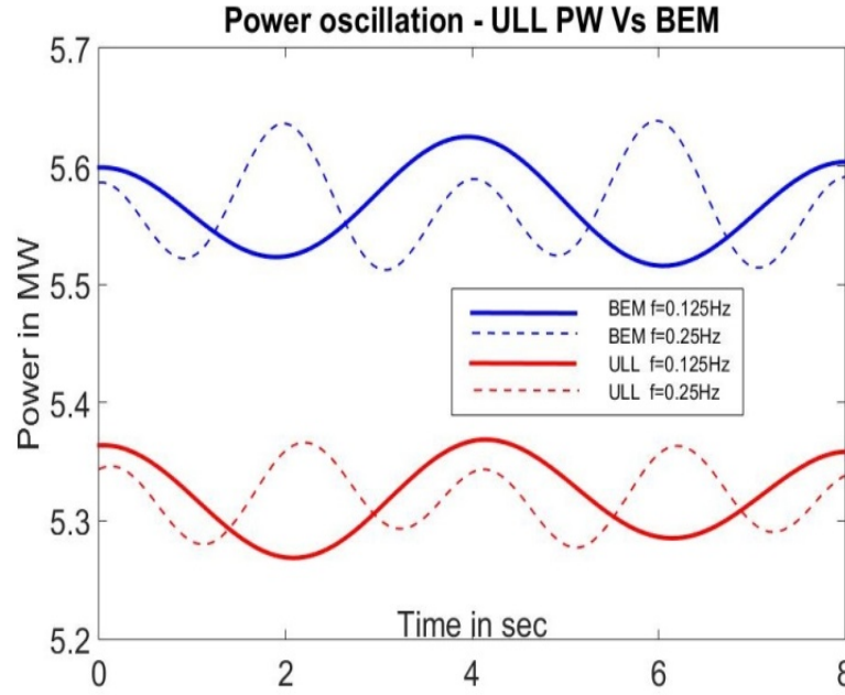
Fig. 5 Comparative diagram of power oscillation for the 20% tip swept NREL 5MW rotor predicted by ULL and BEM. Amplitude = 12deg - frequency = 0.125 and 0.25Hz - t=0 tip starts with aft sweep.
