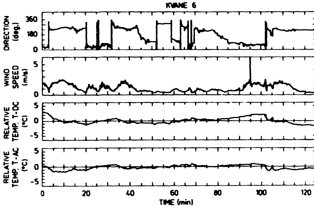
Fig.6.2. Measurements at the valley mast of the fluctuating wind speed, wind direction and temperature for the experiment on August 10, 1981. The temperature stated as T-DC are bandpass filtered with an upper frequency that can be characterized by a time constant of 1 s and a lower frequency of roughly 75 min; the temperature stated T-AC are filtered with an identical lowpass filter but the highpass filter are characterized by a time constant of 10 min. Downwind flow corresponds to a wind direction of approximately 60 deg, upwind to about 240 deg. The record starts at 0220 local time.
