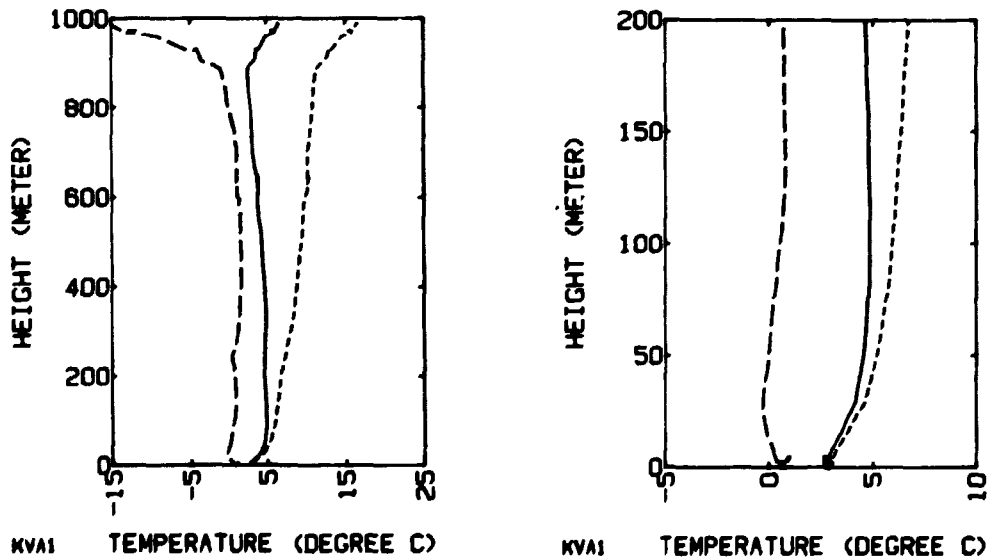
Fig.1.3. Vertical profiles of potential temperature, temperature and dew point temperature up to 1000 and 200 meter respectively for the experiment on July 26, 1981. The radiosonde was released at the Dyrnes camp more than 1 hour after the experiment.
