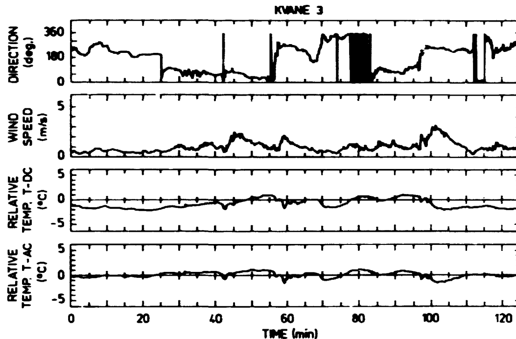
Fig.3.1. Measurements at the valley mast of the fluctuating wind speed, wind direction and temperature for the experiment on August 1, 1981. The temperature stated as T-DC are bandpass filtered with an upper frequency that can be characterized by a time constant of 1 s and a lower frequency of roughly 75 min; the temperature stated T-AC are filtered with an identical lowpass filter but the highpass filter are characterized by a time constant of 10 min. Downwind flow corresponds to a wind direction of approximately 60 deg, upwind to about 240 deg. The record starts at 0140 local time.
