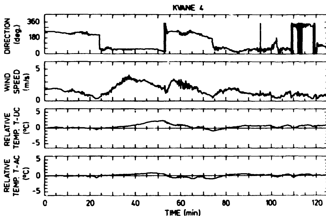
Fig. 4.2. Measurements at the valley mast of the fluctuating wind speed, wind direction and temperature for the experiment on August 4, 1981. The temperature stated as T-DC are bandpass filtered with an upper frequency that can be characterized by a time constant of 1 s and a lower frequency of roughly 75 min; the temperature stated T-AC are filtered with an identical lowpass filter but the highpass filter are characterized by a time constant of 10 min. Downwind flow corresponds to a wind direction of approximately 60 deg, upwind to about 240 deg. The record starts at 0330 local time.
