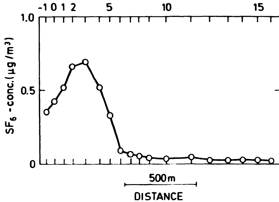
Fig.6.1. Experiment 10 August, 1981; (KVANE 6). Mean values, averaged over 1 hour, of the measured tracer concentrations. The positions have been projected on a line perpendicular to the direction R-position 3 in Fig.1.
