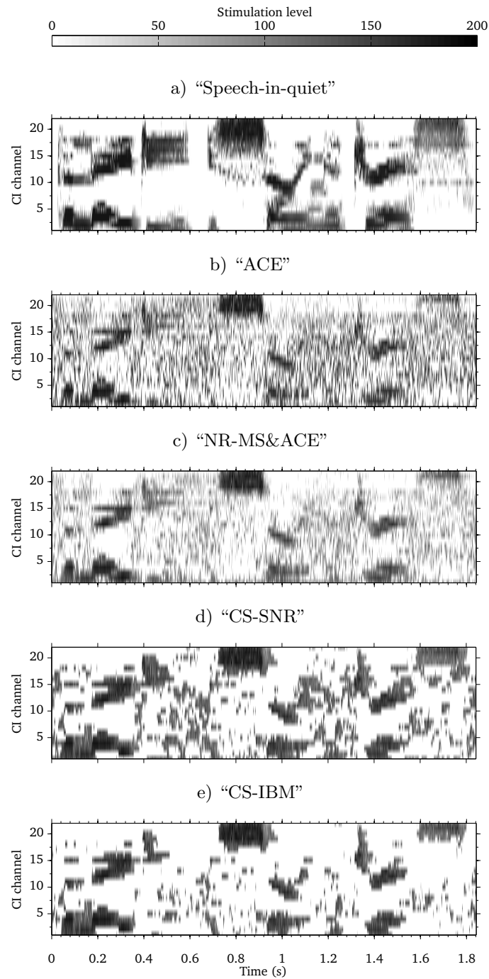
Figure 4.7: The ideal electrodiagram ("Speech-in-quiet") was obtained by processing the speech signal with ACE. In Figs. 4.7b-e, the speech signal was mixed with speech-weighted noise at 0 dB SNR and processed with the four strategies in Session 1. Graytones correspond to a stimulation level between the T and C level.
