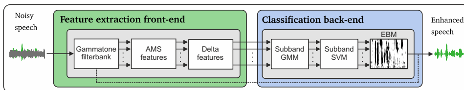
Figure A.1: Block diagram of the segregation system that shows the main blocks of the feature extraction front-end and the classification back-end. The dashed line illustrates the reconstruction of the target by applying the EBM to the subband signals of the noisy speech.
