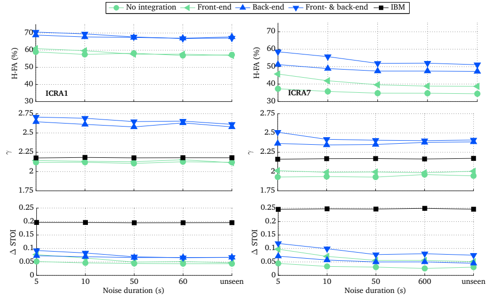
Figure A.2: H-FA, \gamma and STOI improvements for the four models and the IBM averaged across 180 sentences and SNRs ( -5 and 0 dB) for ICRA1 (left panels) and ICRA7 (right panels). Average STOI values of the unprocessed noisy speech were 0.66 (ICRA1) and 0.63 (ICRA7).
