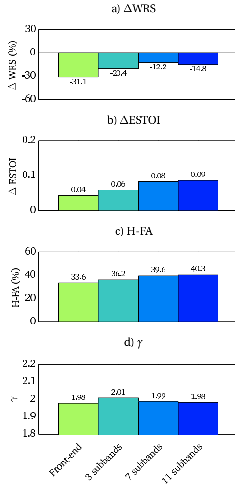
Figure 2.6: Experiment II's \Delta WRS relative to noisy speech (first row of panels), \Delta ESTOI relative to noisy speech (second row of panels), H-FA rates (third row of panels) and \gamma values (fourth row of panels) with the four different system configurations in ICRA7. WRS improvements are derived from the Paired Student's t-tests and significant improvements (on a 5% significance level) are marked with an asterisk (*). All objective measures are evaluated at -5 dB SNR.
