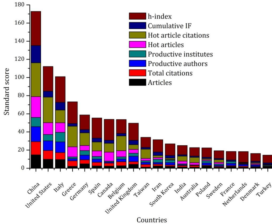
Figure 4: Standard research output score of the most productive countries
