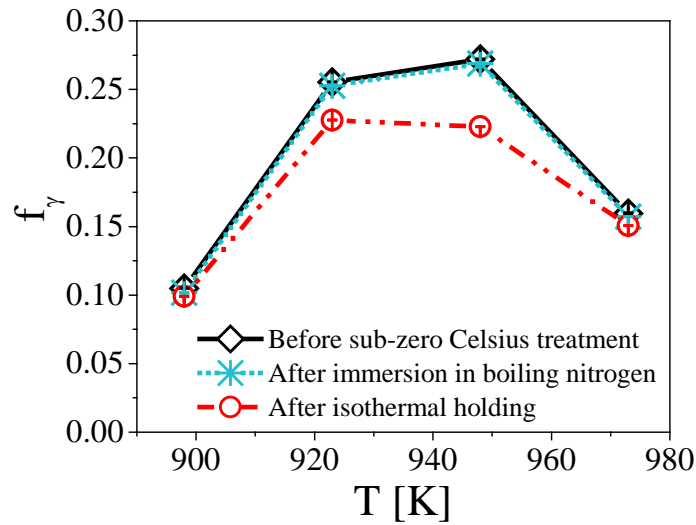
Figure 2. Fraction of austenite f_{\gamma} versus annealing temperature T . The three data sets refer to the material before sub-zero Celsius treatment, after immersion in boiling N 2 for 0.3 ks and after additional isothermal holding at 195 K for 15.3 ks.
