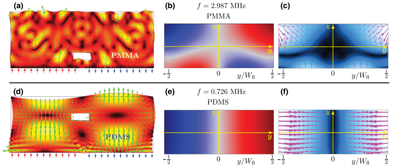
FIG. 9. Numerical results for the PMMA device [(a)–(c)] and a corresponding PDMS device with its cavity displaced 0.5 mm upward [(d)–(f)]. (a) The displacement field \mathbf{u} (green arrows) and its magnitude (color plot) from 0 nm (black) to 10 nm (white) in the PMMA device as in Fig. 6 but for the higher resonance f_7 = 2.987 MHz of Q = 109 . To be visible, the nanometer-scale displacement has been increased by a factor of 5000. (b) Color plot of the corresponding pressure field p_1 in the water from -210 kPa (blue) to 210 kPa (red). (c) The corresponding radiation force \mathbf{F}^{\text{rad}} (magenta arrows) on a 10\text{-}\mu\text{m} -diameter spherical polystyrene tracer particle and its magnitude (color plot) from 0 pN (black) to 1.9 pN (light yellow) as a function of its position in the water. (d) As for (a) but for a PDMS device at the low resonance 0.726 MHz of Q = 122 and with the displacement magnitude u from 0 nm (black) to 19 nm (light yellow). (e) The pressure field p_1 as in (b) but with higher amplitude 310 kPa. (f) The radiation force \mathbf{F}^{\text{rad}} as in (c) but with lower amplitude 0.3 pN.
