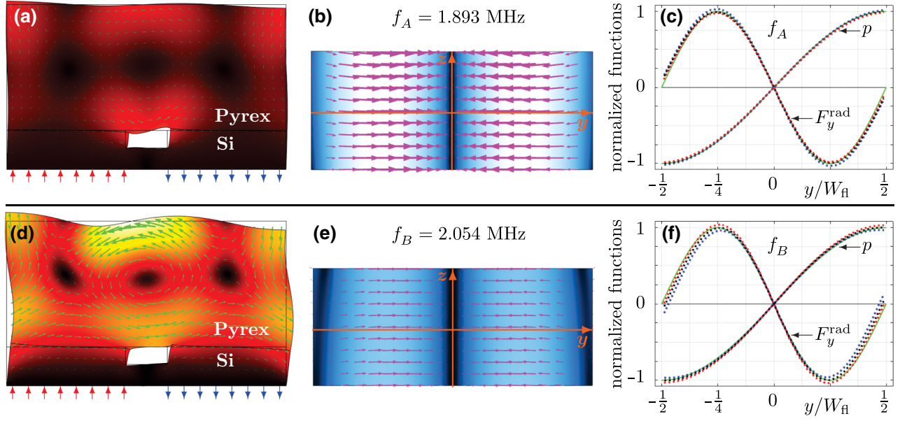
FIG. 4. Numerical results for resonances A and B in Fig. 3 of the glass-silicon device. (a)–(c) are for f_A = 1.893 MHz. (a) Vector plot in the solid domain \Omega_{sl} of the displacement field \mathbf{u} (green arrows) and color plot of its amplitude u from 0 nm (black) to 2.6 nm (white). To be visible, the nanometer-scale displacement has been increased by a factor of 50 000. (b) The radiation force \mathbf{F}^{\text{rad}} on a 10- \mu\text{m} -diameter spherical polystyrene tracer particle as a function of its position in the fluid domain \Omega_{fl} . Color plot of the magnitude F^{\text{rad}} from 0 pN (black) to 11.5 pN (white) and vector plot (magenta arrows) of \mathbf{F}^{\text{rad}} . (c) Comparison of the numerical simulation of the silicon-glass device (dotted lines) in Fig. 3 with the analytical result for the hard-wall device (solid green line). The normalized pressure p/p_{\text{norm}} (half-wave, p_{\text{norm}} = 209 kPa) and y component of the radiation force F_y^{\text{rad}}/F_{\text{norm}}^{\text{rad}} (full wave, F_{\text{norm}}^{\text{rad}} = 11.0 pN) plotted along the top, center, and bottom horizontal lines at z = 0.9H_{fl} (blue dots), z = 0.5H_{fl} (black dots), and z = 0.1H_{fl} (red dots), respectively. (d),(e),(f) are as (a),(b),(c), respectively, but for f_B = 2.054 MHz with p_{\text{norm}} = 138 kPa and F_{\text{norm}}^{\text{rad}} = 5.05 pN.
