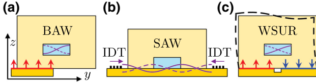
FIG. 1. The conventional and proposed acoustophoresis techniques for a liquid-filled microchannel (blue) embedded in an elastic solid (beige). (a) BAWs excited by a single piezoelectric actuator (orange). (b) SAWs excited by interdigitated transducers (IDT; black) on a piezoelectric substrate (orange). (c) The proposed WSURs excited by two piezoelectric actuators excited in antiphase (red and blue arrows). Magenta and dashed black curves represent pressure and displacement fields, respectively.
