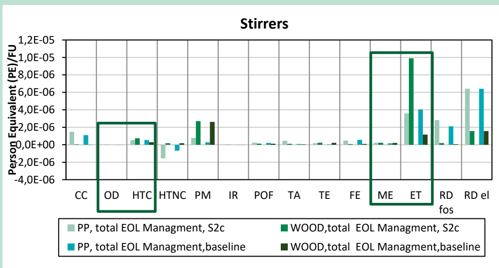
FIGURE 13. Normalized potential impacts for Scenario Sensitivity S2c (i.e. 100% heat from wood) for Stirrers, in comparison to baseline results. . Acronyms for impact categories are explained in Table 4.
