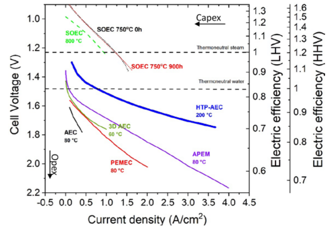
Figure 2. Cell voltage versus current densities for various types of electrolysis technologies applicable for the production of hydrogen by water/steam splitting. Right-hand scales illustrate the achievable efficiencies
