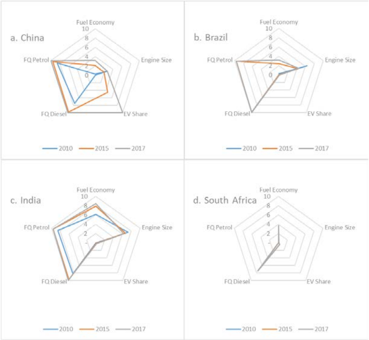
Figure 3. Trends in fuel economy, fuel quality, engine size and electrification Values are normalized on a scale of 0 to 10. A score of 10 is given for a fuel economy of 5 liter per 100 km, engine size of 1100 cc, EV market share of 2.2%, FQ diesel of 10 ppm of sulphur and FQ petrol of 10 ppm of sulphur. Source: for Fuel Economy and Engine Size data from [6] for Electrification from [7]
