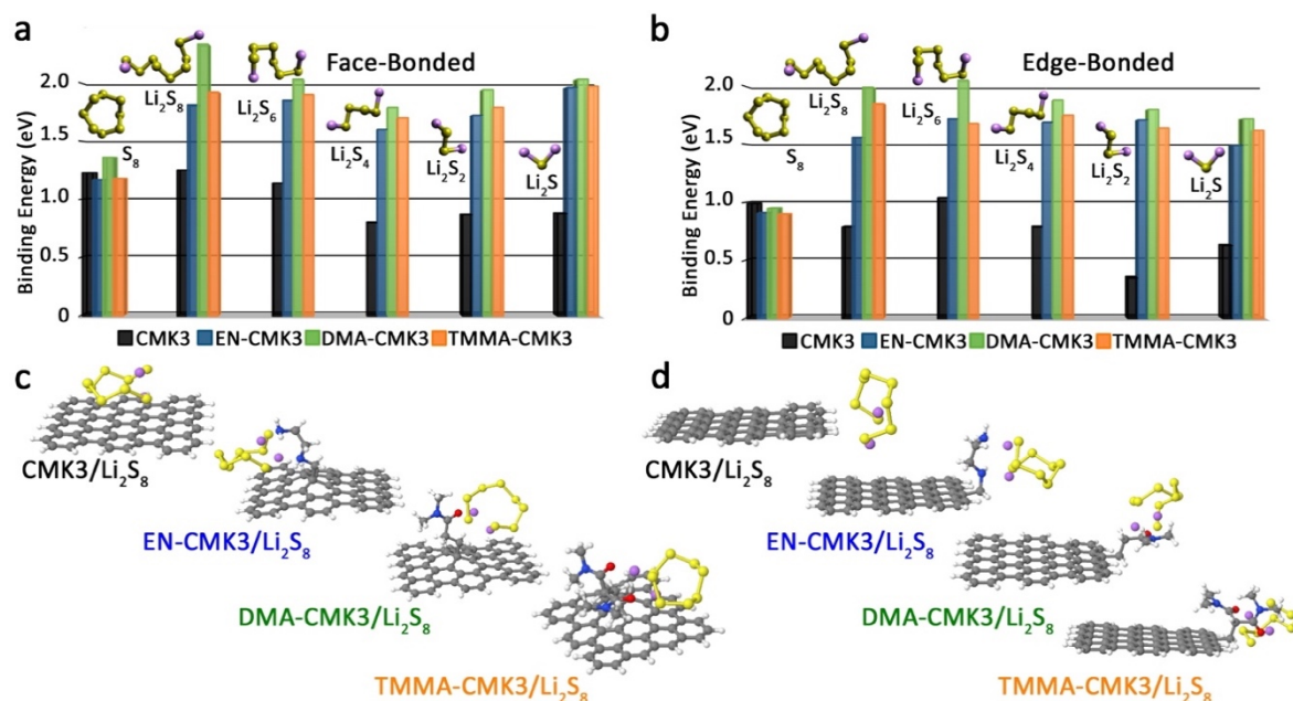
Figure 3. Binding energies between different sulfur species and an unfunctionalized (CMK3) or functionalized (EN-CMK3, DMA-CMK3, TMMA-CMK3) surface. Functional groups are either a face-bonded or b edge-bonded. Optimized structures between the surface and \text{Li}_2\text{S}_8 are shown for c face-bonded and d edge-bonded groups.
