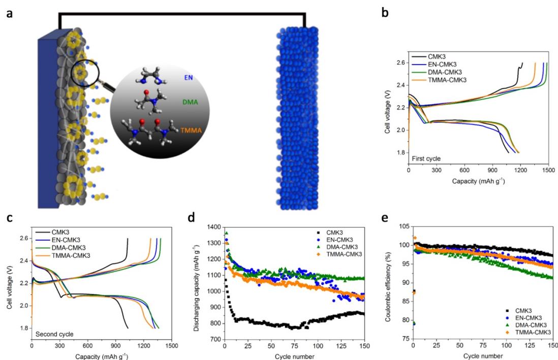
Figure 4. Battery configuration and galvanostatic cycling performance of Li-S cells using CMK3 cathodes cycled between 1.8 – 2.6 V at a rate of C/10 (167.5 mA g -1 ). a Li-S battery configuration including the use of functionalized CMK3. b Voltage profiles for the 1 st cycle and c 2 nd cycle. d and e Specific discharging capacities versus cycle number.
