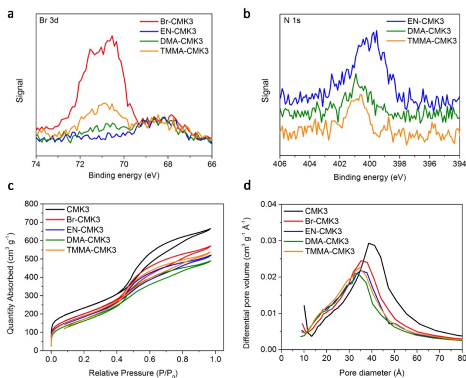
Figure 2. Characterization of the functionalized CMK3. X-ray photoelectron spectra (XPS) of the a Br 3d and b N 1s regions. In the N 1s spectra, the plots have been offset in signal intensity for clarity. c Nitrogen adsorption-desorption isotherms and d corresponding pore size distributions based on the adsorption isotherm.
