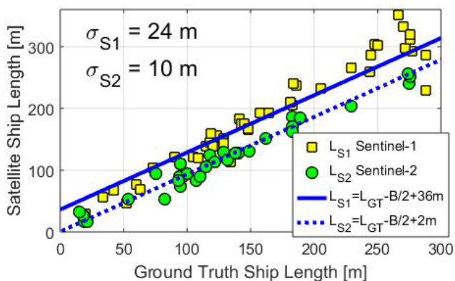
Figure 6. Ship lengths. Squares and circles are from S1 and S2 data respectively vs ground truth lengths and breadths from AIS ship records. Blue lines indicate best off-set fit to S1 data and dashed blue line to S2 data, see text.
