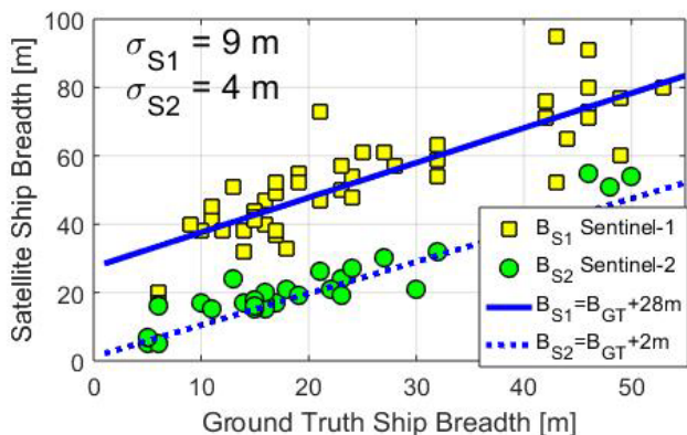
Figure 7. As Fig. 6 but for ship breadths.
