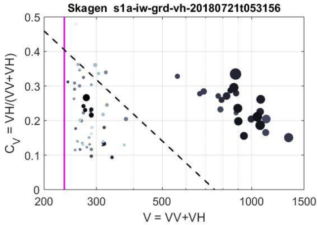
Figure 5. As Fig. 4 but for all segments (mainly ships, sidelobes and wakes) found in Fig. 2 of Skagen. Dashed line is the k-nearest-neighbor (kNN) classification decision boundary.
