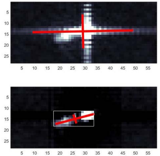
Figure 3. Top: S1 SAR image of the container ship Ivar Reefer in Fig.2. Ship dimensions are 164x26m but show strong sidelobes. Bottom: sidelobes have been removed. Red bars show the resulting and improved ship length, breadth and direction.
