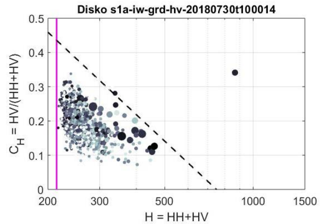
Figure 4. Scatter plots of all segments (mainly icebergs) found in the Disko Bay ROI of Fig.1. Backscatter distribution C_H vs. H , where size is proportional to area A and shading to B/L . This gives a visual view of the four classification parameters. Vertical line is the threshold T_B . Almost one thousand icebergs and ice floes are correctly classified below the dashed line. According to AIS there are two ships present of which the large cruise ship Ocean Diamond is clearly separated on the right whereas a smaller trawler is not identified.
