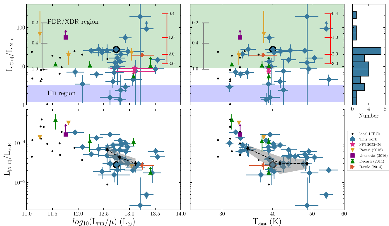
Figure 3. Comparison of key properties of our lensed sample of [N\text{ II}] and [C\text{ II}] observations (shown in blue diamonds) with literature measurements. Top panels: Observed L_{[C\text{ II}]} / L_{[N\text{ II}]} plotted against demagnified L_{\text{FIR}} and dust temperature. Expected L_{[C\text{ II}]} / L_{[N\text{ II}]} regimes for H II and photon or x-ray dominated regions based on Decarli et al. (2014) are shown. Modelled metallicity grids for ISM densities of \log(n) = 1.5 (grey) and 3.0 (red), each with ionization parameter \log(U_{\text{H II}}) = -3.5 , are shown as floating axes (Nagao et al. 2012) with metallicity units of Z/Z_{\odot} . Bottom panels: Observed L_{\text{FIR}} normalized [N\text{ II}] luminosities and dust temperature. For literature sources, the upwards green triangles represent sources from Decarli et al. (2014): two Lyman alpha emitters, an SMG, and a quasar in order of increasing L_{\text{FIR}} at z = 4.7 . The downwards yellow triangles represent Pavesi et al. (2016) sources, which are LBG-1 (typical Lyman-break galaxy), HZ10 (FIR-luminous LBG), and AzTEC-3 (a massive SMG) in order of increasing L_{\text{FIR}} at z = 5.3\text{--}5.65 . The purple square represents LAB1-ALMA3, a galaxy embedded in a Lyman alpha blob at z = 3.1 (Umemata et al. 2017). A SMG (rightward orange triangle) at z = 5.243 from Rawle et al. (2014) and two components of SPT2052-56, an unlensed protocluster of SMGs at z = 4.3 , are also shown (pink stars – Pass et al., in preparation). SPT2132-58 (B  thermin et al. 2016) has a black circular background. Local LIRGs assembled from Lu et al. (2017), D  az-Santos et al. (2017), and Zhao et al. (2016) are shown as small black dots.
