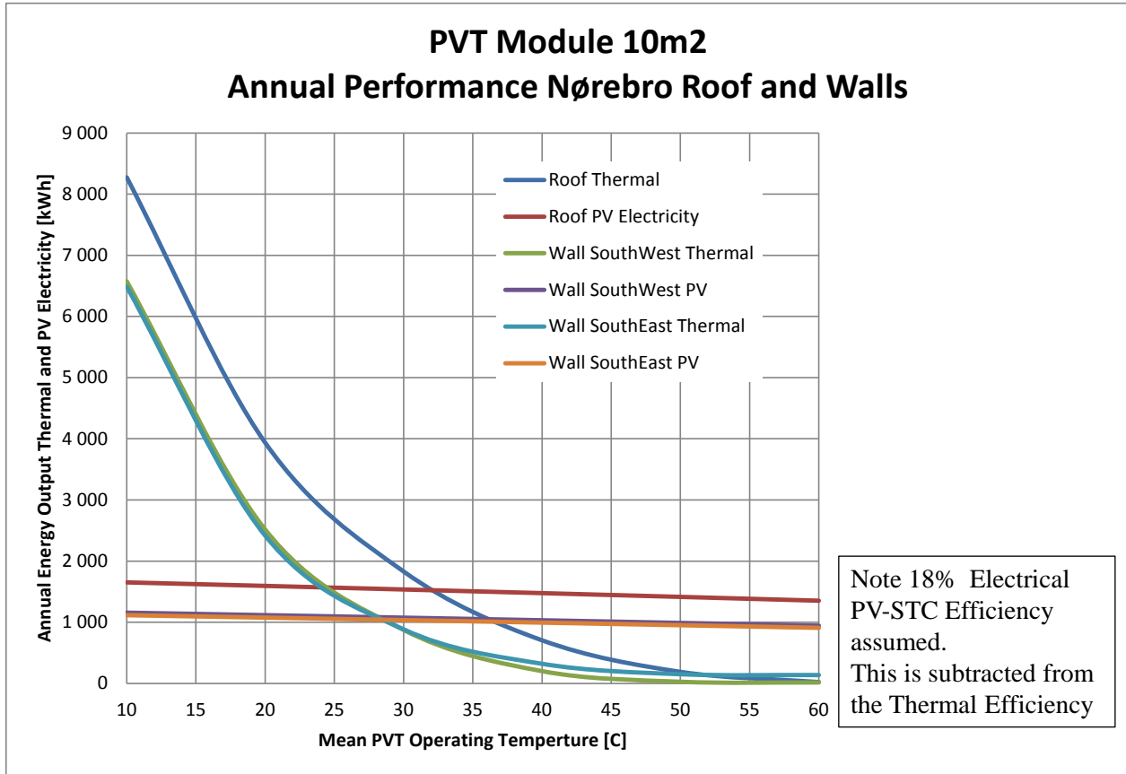
Figure 9. Annual performance, at different operating temperatures. Both electrical and thermal outputs are shown. A 10 m 2 module and 18% STC PV module efficiency is assumed. The calculations are done with the ScenoCalc-PVT tool .
