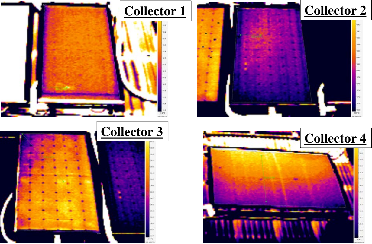
Figure 5. Thermo vision camera pictures indicating that there are no problems with delamination or flow distribution or air enclosures, that can affect the performance results.
