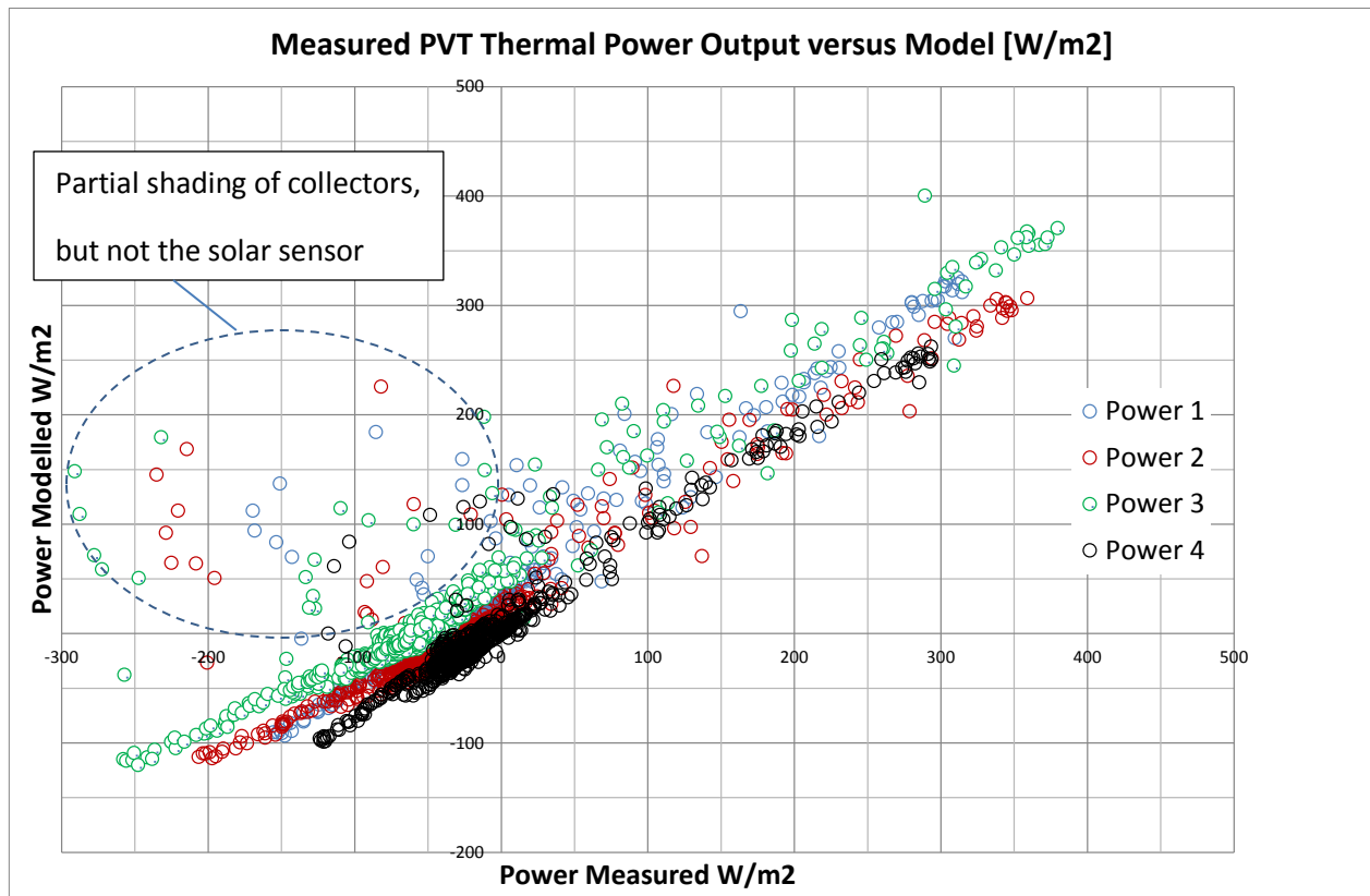
Fig 8. Modelled collector power (Y-axis) versus measured power (X-axis) for collector 1, 2, 3 and 4 for a period in late October with the model and parameters from the July data evaluation. A small difference can be seen between the collectors but it is very close to the measurement accuracy.
