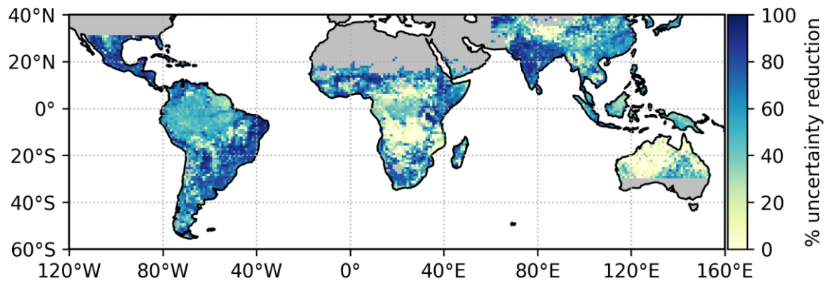
Fig. 8. The relative reduction in the size of the 95% confidence interval of estimated vegetation carbon turnover times when using a prior value for biomass at each pixel compared to a run without a biomass prior. Turnover times were estimated using the CARDAMOM system. The darker areas show where reduction in relative uncertainty is largest.
