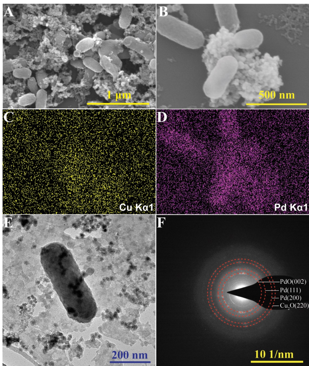
Figure 2. Morphology and composition of S/CuPd-M9_C. (A) SEM image of cells and extracellular NPs. (B) SEM image of Site #2 with four cells and extracellular NPs. (C) Cu EDS mapping and (D) Pd EDS mapping of Site #2. The other elemental mappings are shown in Figure S5 and Figure S6. (E) TEM image of a cell enveloped in EPS with small encapsulated NPs. (F) SAED pattern of extracellular NPs.
