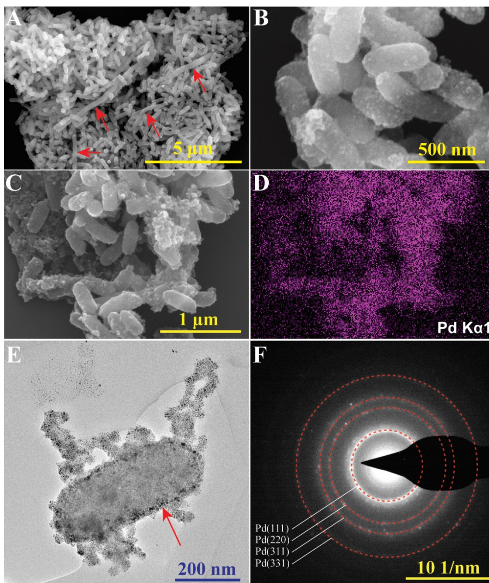
Figure 5. Morphology and composition of S/Pd-NaCl_C. (A) and (B) SEM images at different magnifications. Red arrows in (A) indicate elongated cells. (C) SEM image and (D) corresponding Pd EDS mapping. The other elemental mappings are shown in Figure S16 and Figure S17. (E) TEM image of a cell covered with PdNPs. The red arrow indicates PdNPs accumulation in the periplasm. (F) SAED pattern of NPs associated with cells.
