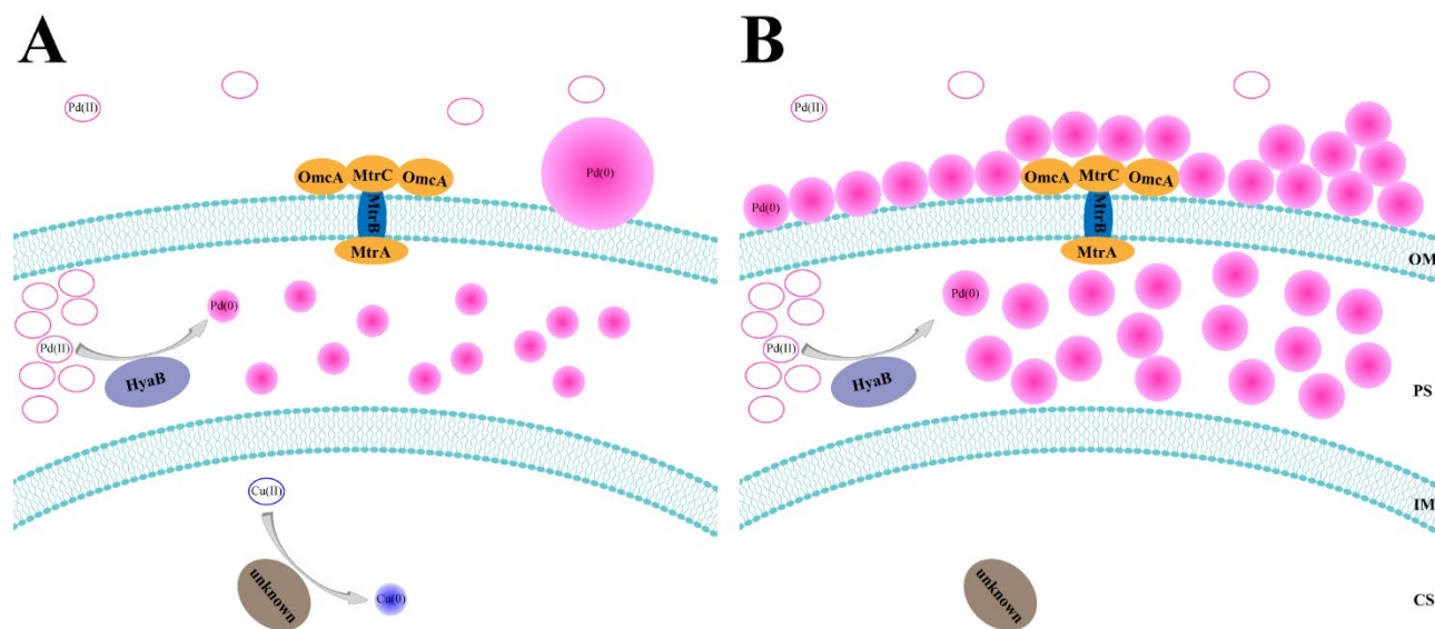
Figure 6. Proposed effect of Cu(II) on the formation of PdNPs. The morphologies and distribution of PdNPs produced by MR-1 incubated in media containing Pd(II) (A) with and (B) without Cu(II). OM: outer membrane; PS: periplasm; IM: inner membrane.
