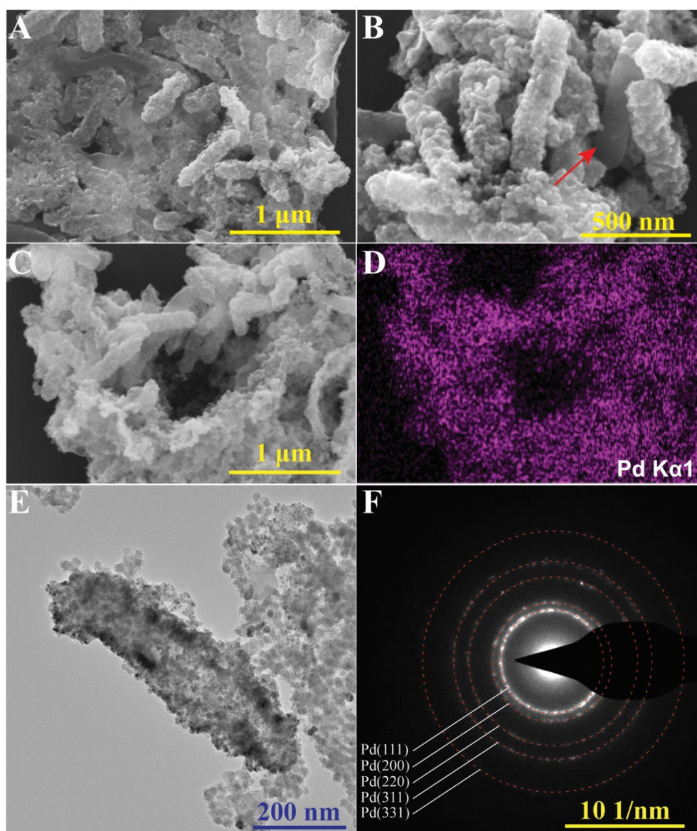
Figure 3. Morphology and composition of S/Pd-M9_C. (A) and (B) SEM images at different magnifications. The red arrow in (B) indicates a cell without PdNP coverage. (C) SEM image and (D) the corresponding Pd EDS mapping. The other elemental mappings are shown in Figure S10 and Figure S11. (E) TEM image of a cell completely covered by PdNPs. (F) SAED pattern of the PdNP coating.
