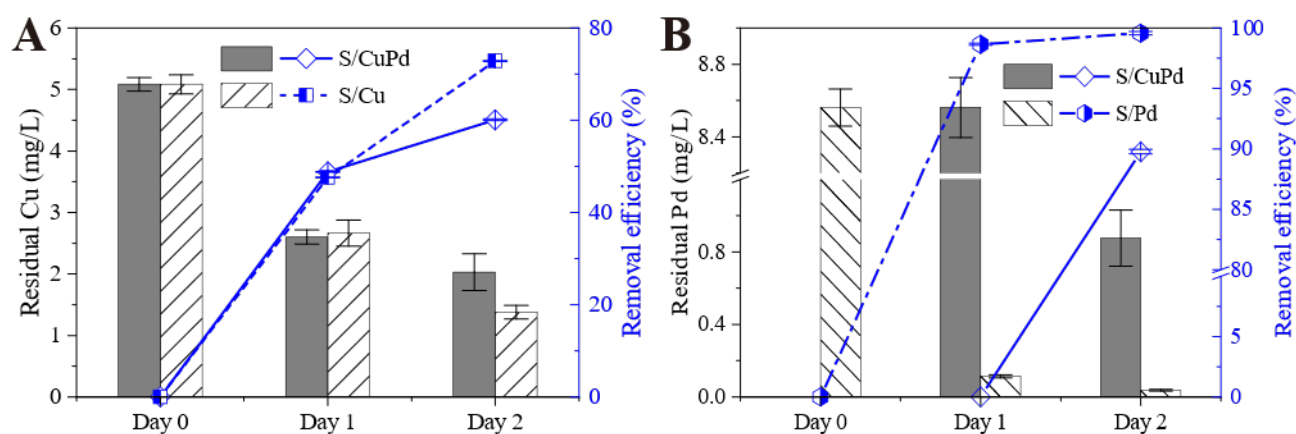
Figure 1. Co-removal of (A) Cu and (B) Pd by MR-1. Residual metals in the medium and corresponding removal efficiency are shown. The error bars indicate the standard deviation from triplicate ( n = 3 ) experiments.
